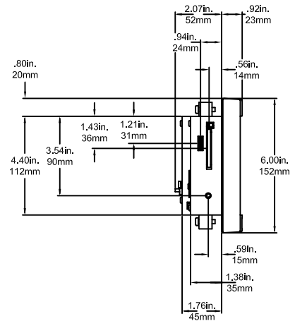
P13 Left Side View
