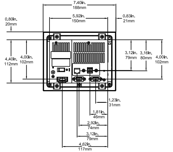
P13 Back View
