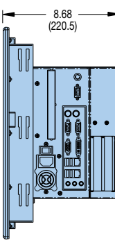
Expansion Chassis Side View
