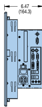
Standard Chassis Side View
