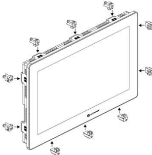
USP-156-xxx: 10 mounting brackets
