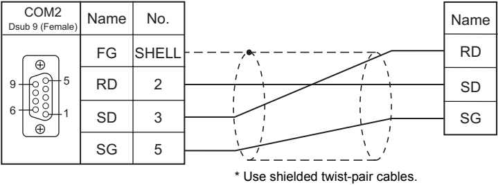
Wiring diagram 2 - COM2
