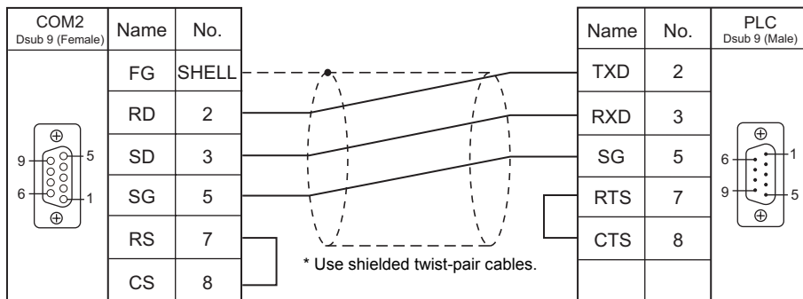
Wiring diagram 8 - COM2
