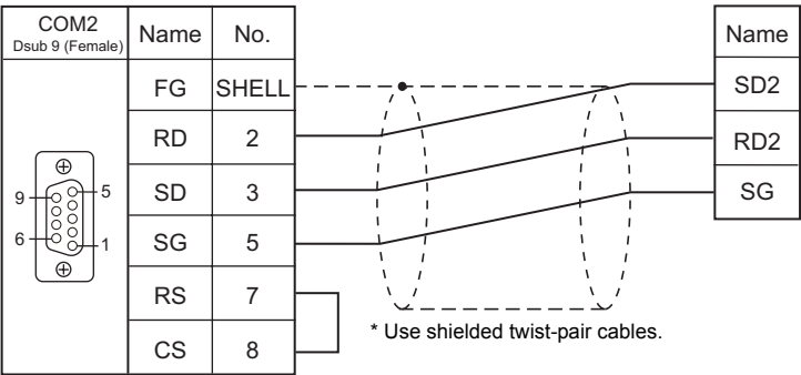
Wiring diagram 3 - COM2
