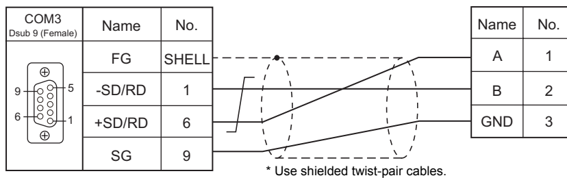
Wiring diagram 3 - COM3
