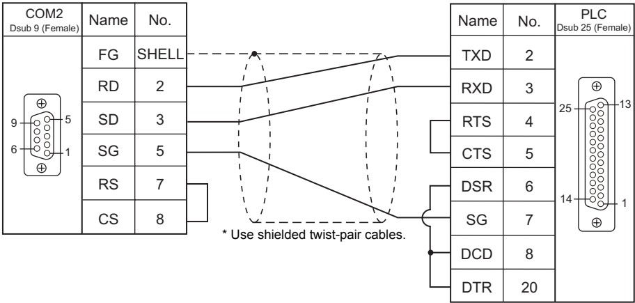
Wiring diagram 4 - COM2
