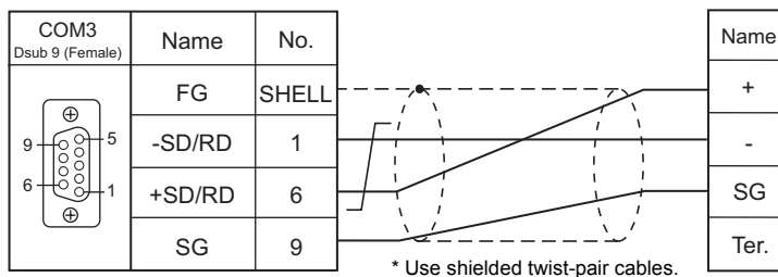
Wiring diagram 15 - COM3
