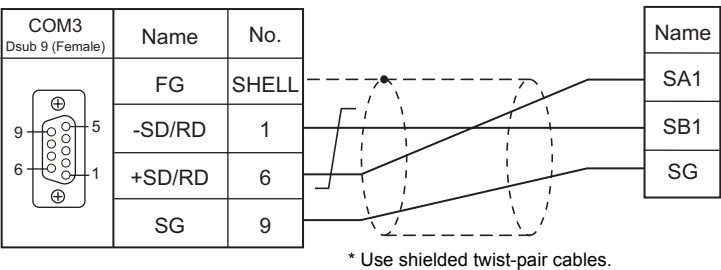
Wiring diagram 2 - COM3
