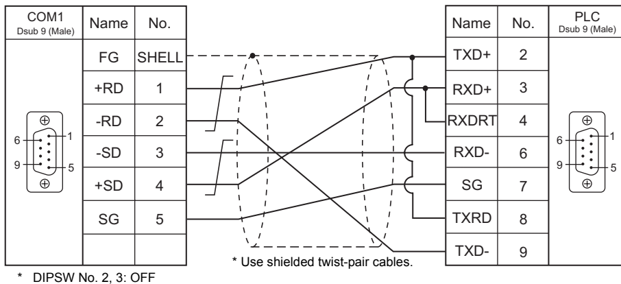
Wiring diagram 3 - COM1
