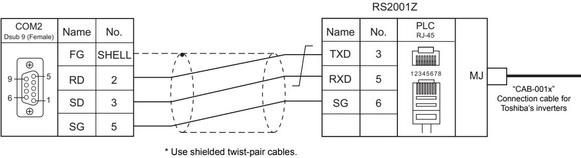
Wiring diagram 1 - COM2
