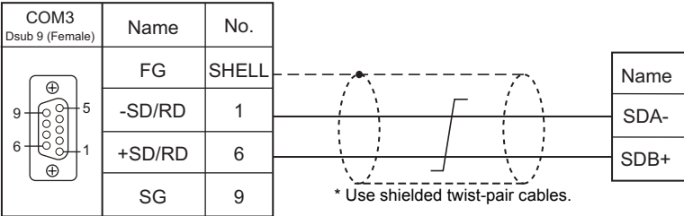
Wiring diagram 1 - COM3
