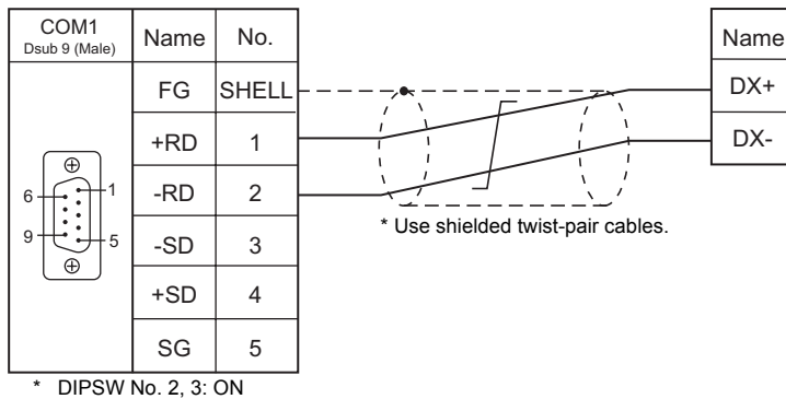
Wiring diagram 8 - COM1
