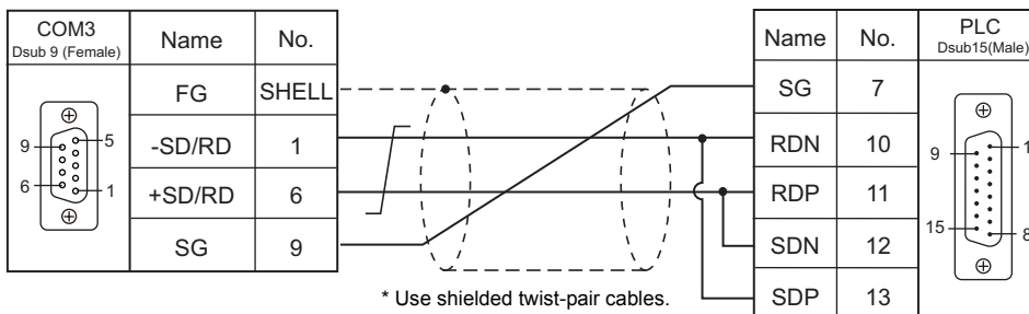
Wiring diagram 4 - COM3
