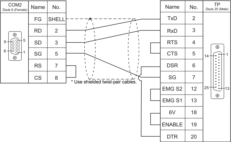
Wiring diagram 3 - COM2
