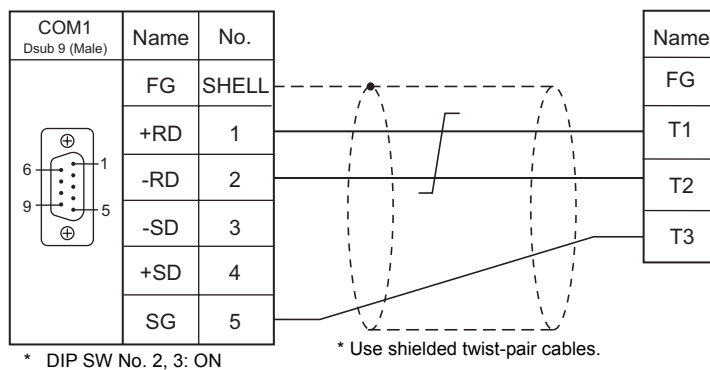
Wiring diagram 6 - COM1
