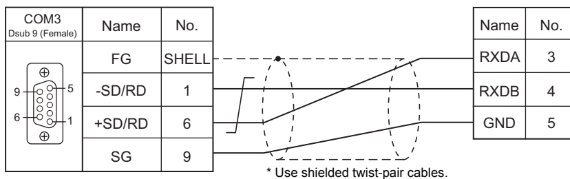
Wiring diagram 4 - COM3
