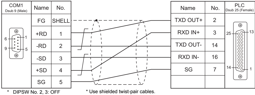
Wiring diagram 3 - COM1
