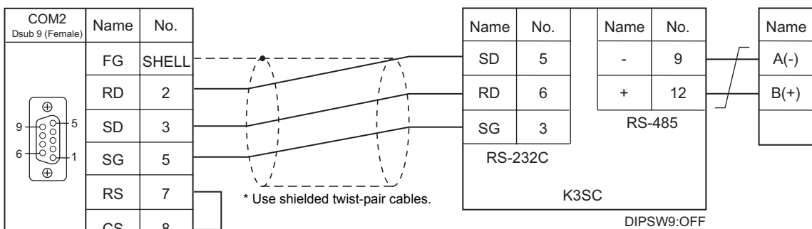
Wiring diagram 4 - COM2
