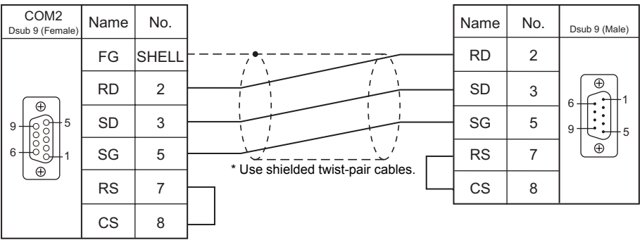
Wiring diagram 5 - COM2
