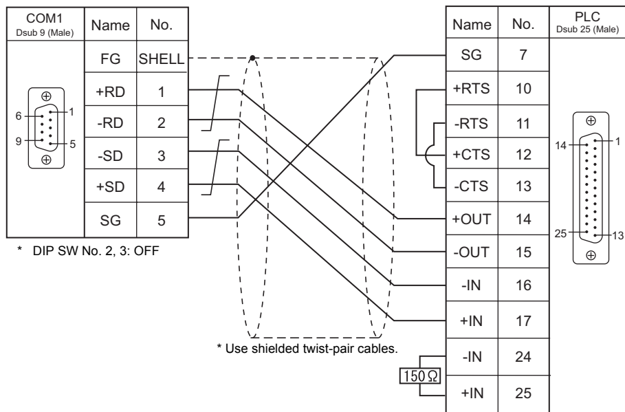
Wiring diagram 5 - COM1
