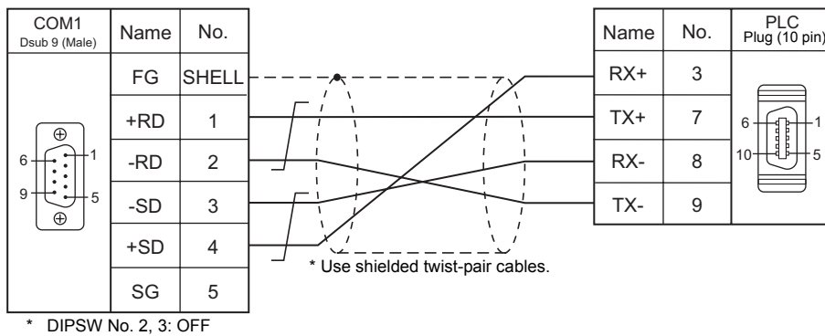
Wiring diagram 10 - COM1
