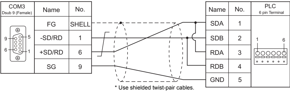
Wiring diagram 4 - COM3
