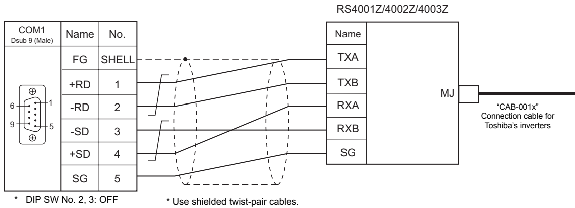
Wiring diagram 1 - COM1
