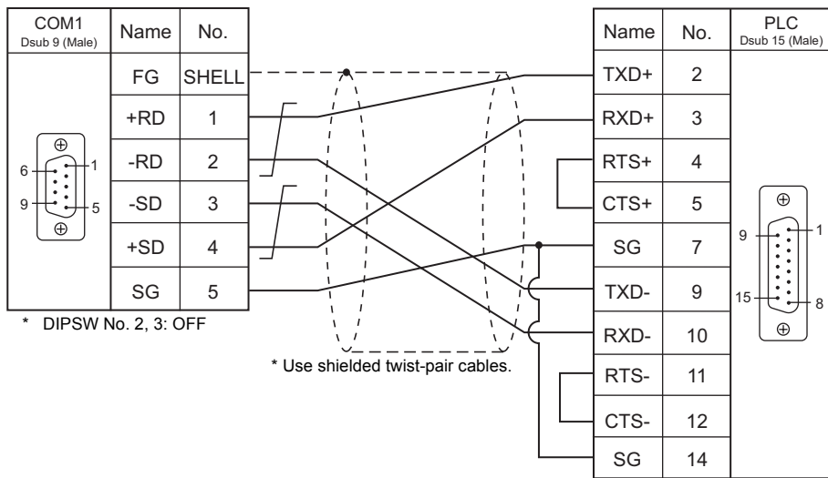
Wiring diagram 5 - COM1
