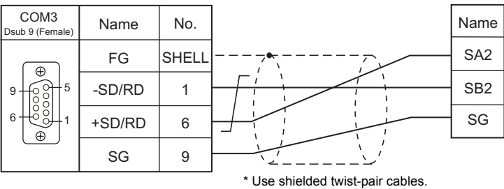
Wiring diagram 3 - COM3
