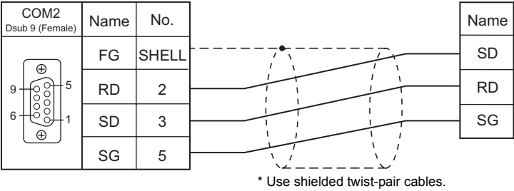
Wiring diagram 1 - COM2
