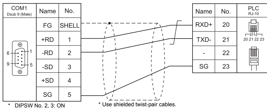
Wiring diagram 11 - COM1
