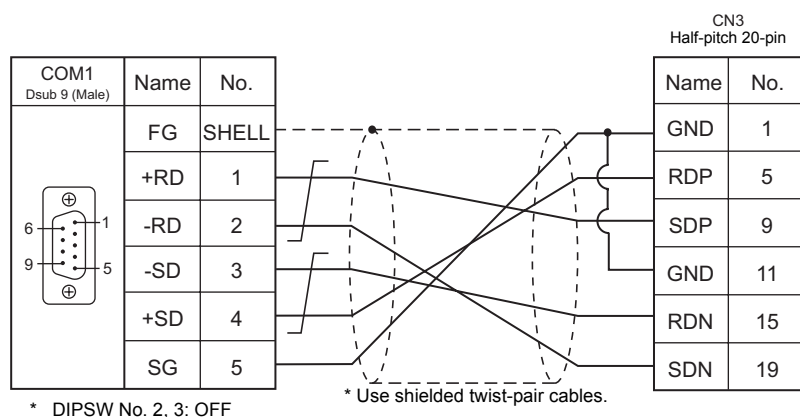
Wiring diagram 2 - COM1
