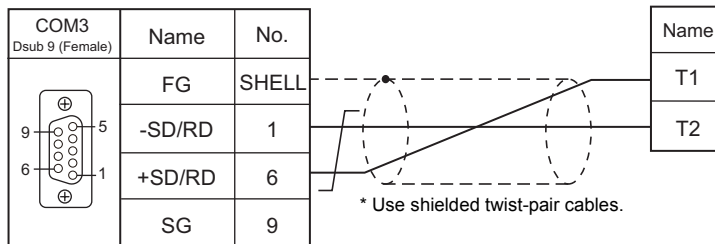
Wiring diagram 13 - COM3
