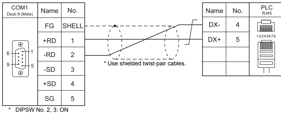
Wiring diagram 10 - COM1
