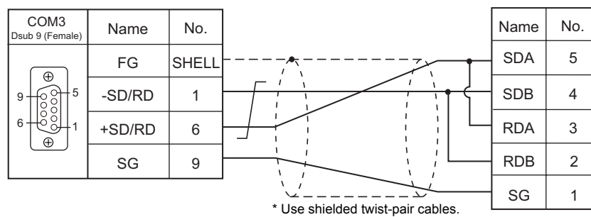
Wiring diagram 4 - COM3
