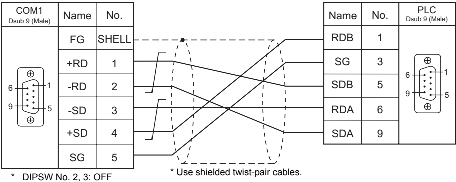
Wiring diagram 4 - COM1
