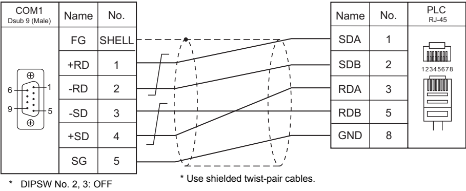
Wiring diagram 4 - COM1
