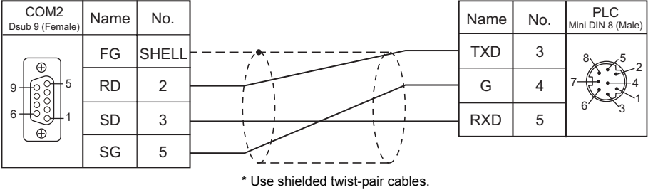
Wiring diagram 3 - COM2
