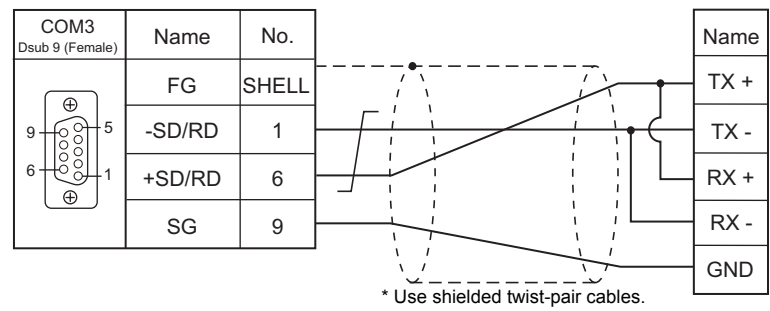
Wiring diagram 1 - COM3
