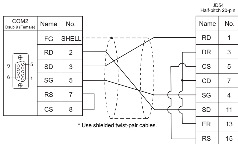
Wiring diagram 3 - COM2
