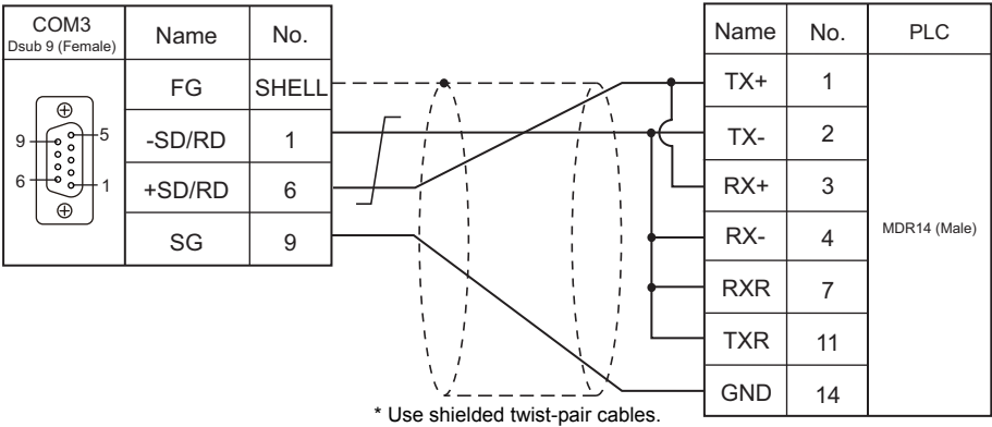
Wiring diagram 5 - COM3
