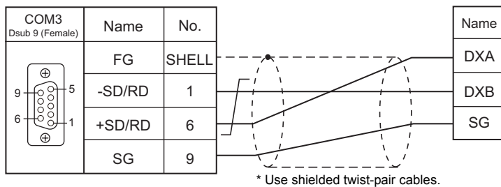
Wiring diagram 4 - COM3
