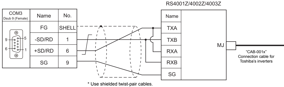
Wiring diagram 1 - COM3
