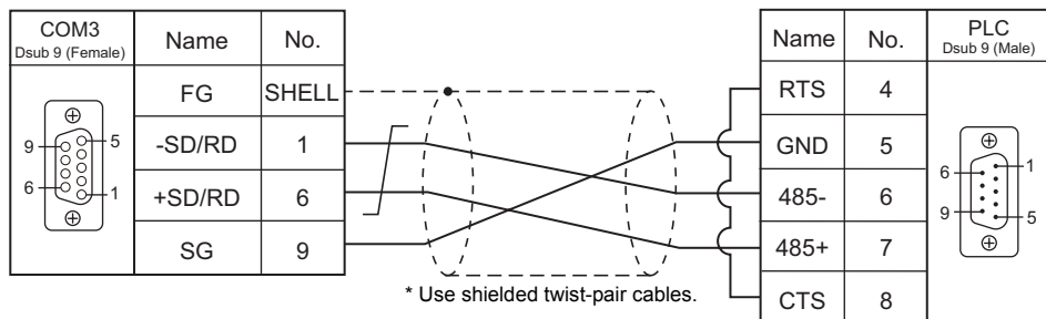
Wiring diagram 2 - COM3
