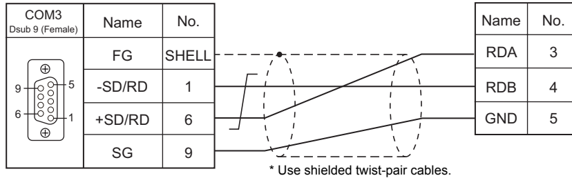
Wiring diagram 1 - COM3
