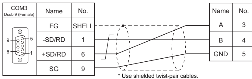
Wiring diagram 2 - COM3
