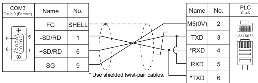
Wiring diagram 14 - COM3
