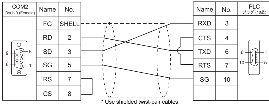
Wiring diagram 6 - COM2
