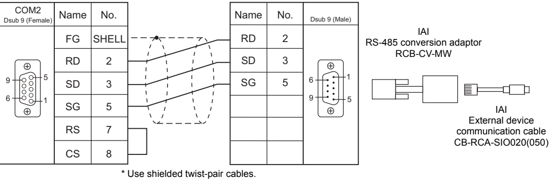
Wiring diagram 3 - COM2
