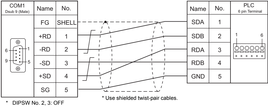
Wiring diagram 5 - COM1
