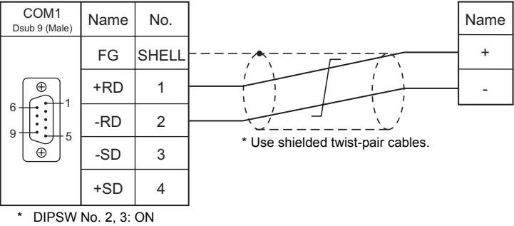
Wiring diagram 1 - COM1
