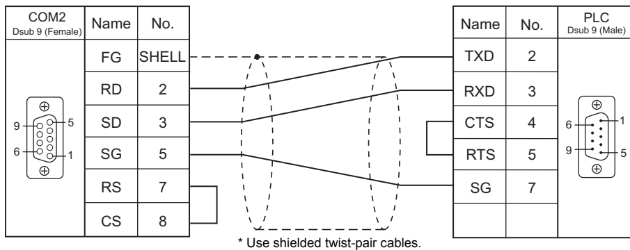
Wiring diagram 7 - COM2
