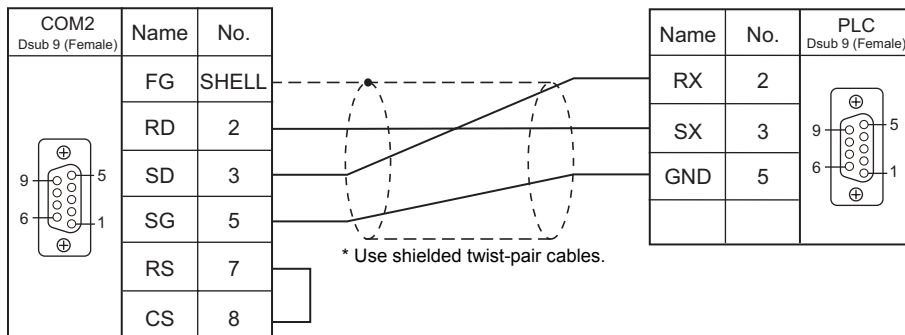
Wiring diagram 9 - COM2
