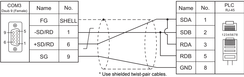
Wiring diagram 3 - COM3
