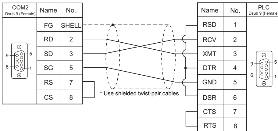
Wiring diagram 5 - COM2
