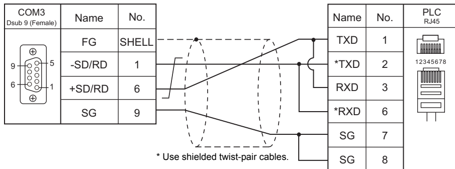
Wiring diagram 13 - COM3
