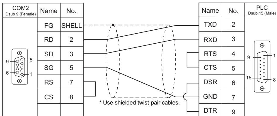
Wiring diagram 3 - COM2
