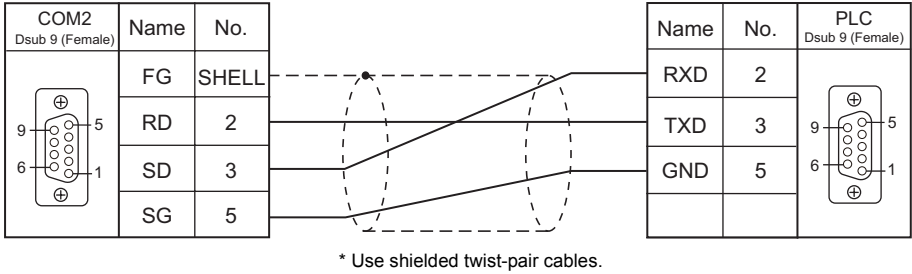
Wiring diagram 1 - COM2
