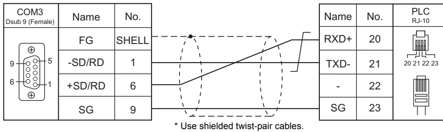
Wiring diagram 12 - COM3
