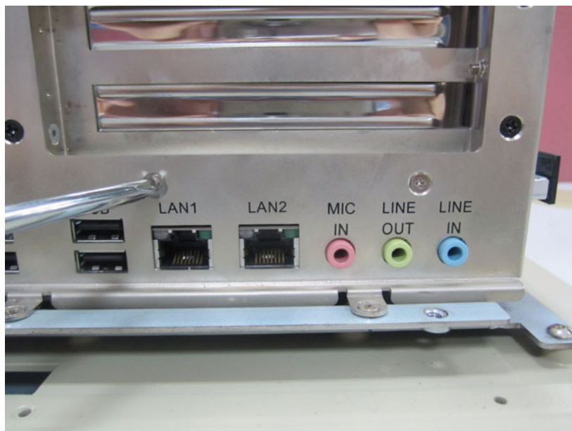
Figure 4.13 I/O Shielding
