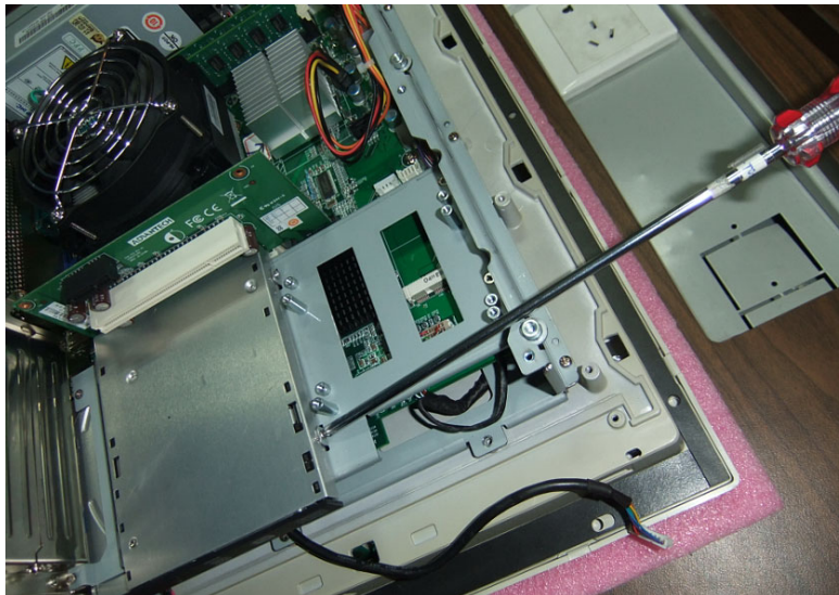
Figure 4.12 Rear Cover Photo with ODD Bracket
