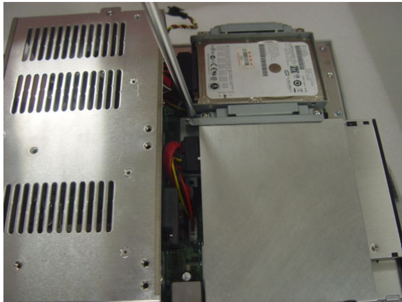
Figure 4.13 Rear Cover Photo with ODD Bracket
