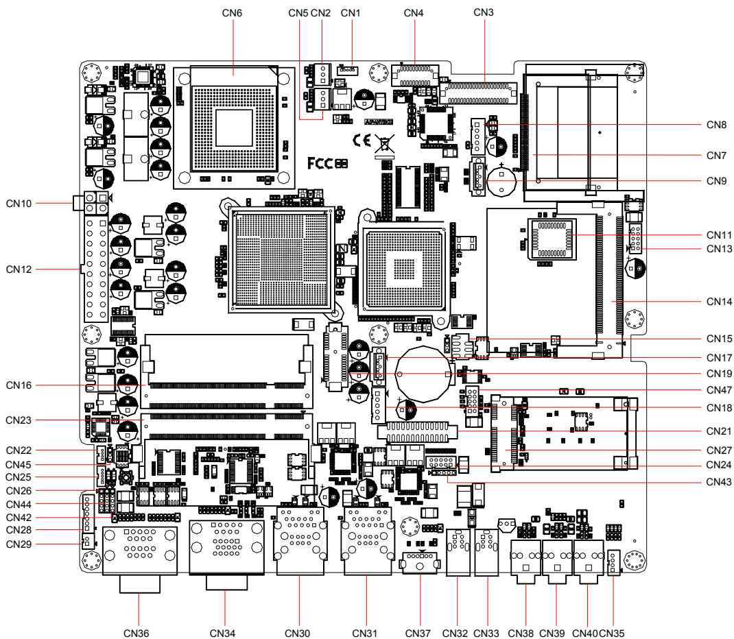
Figure 5.1 Jumpers & Connectors on PPC-157T Motherboard
