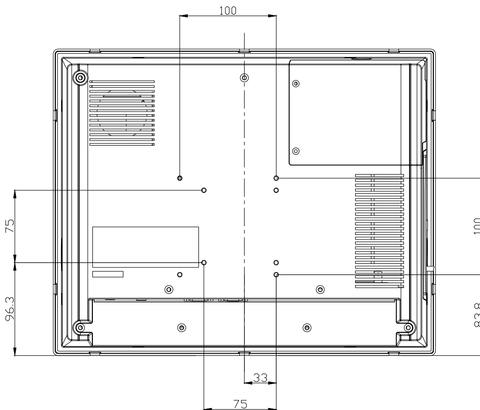
Figure 2.4 Rear View of the Panel PC
