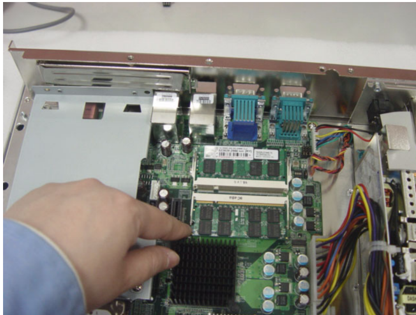
Figure 4.11 Placing the Memory Module in the SODIMM Socket
