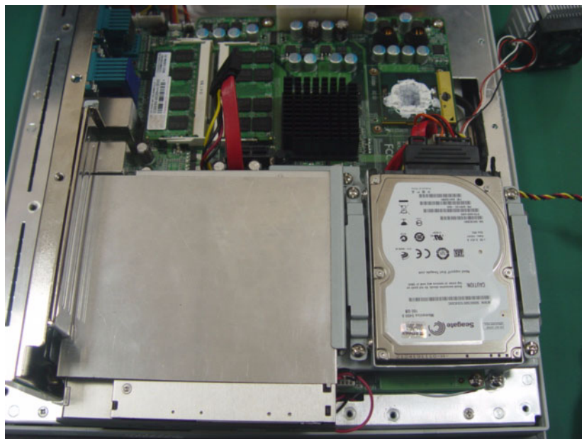
Figure 4.6 Plugging in the SATA Cable
