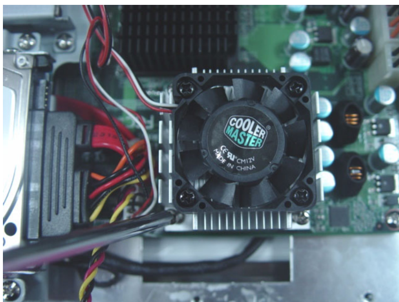
Figure 4.7 Placing the Heatsink and FAN on CPU, then Fastening
