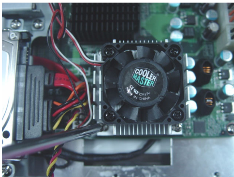
Figure 4.10 Placing the Heatsink and Fan on the CPU, then Fastening
