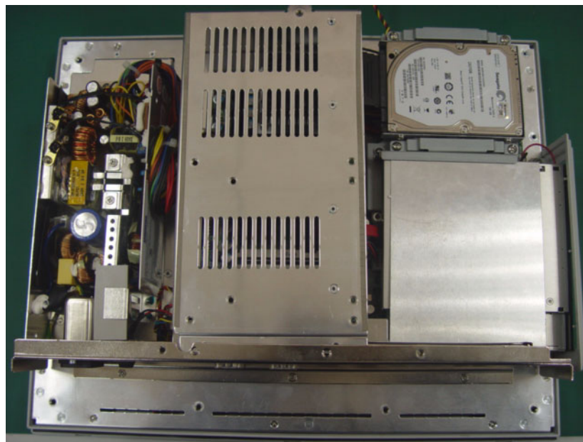
Figure 4.3 The PPC without the Rear Cover
