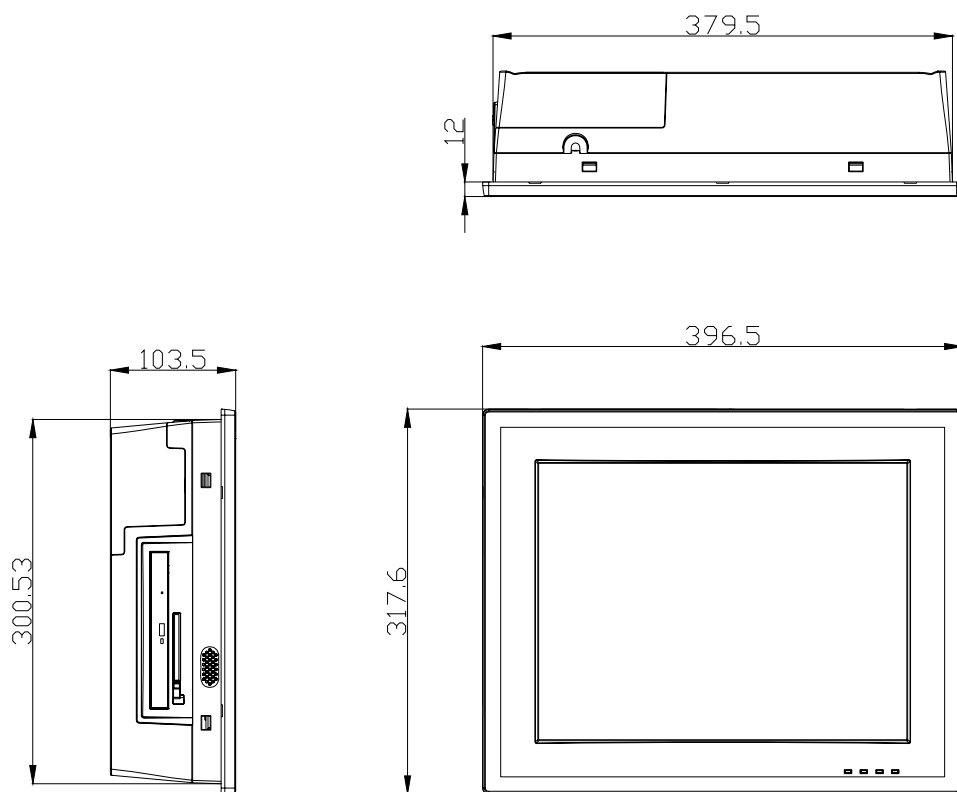
Figure 1.1 Dimensions of PPC-157T
