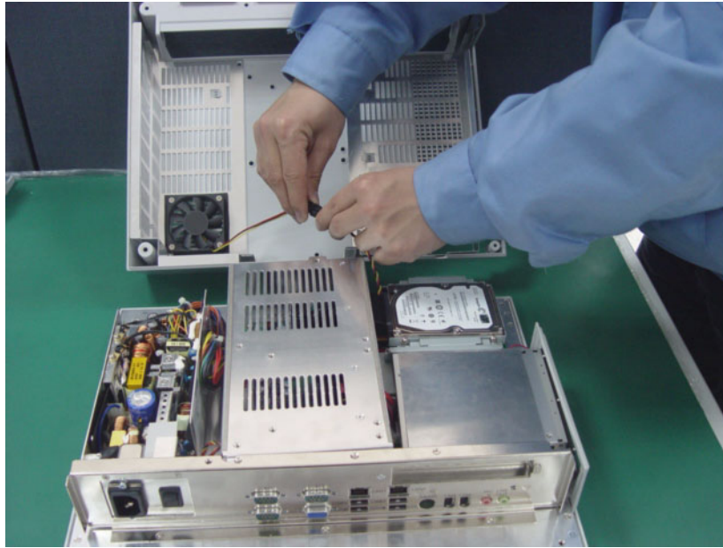
Figure 4.2 Disconnecting the Fan Connector
