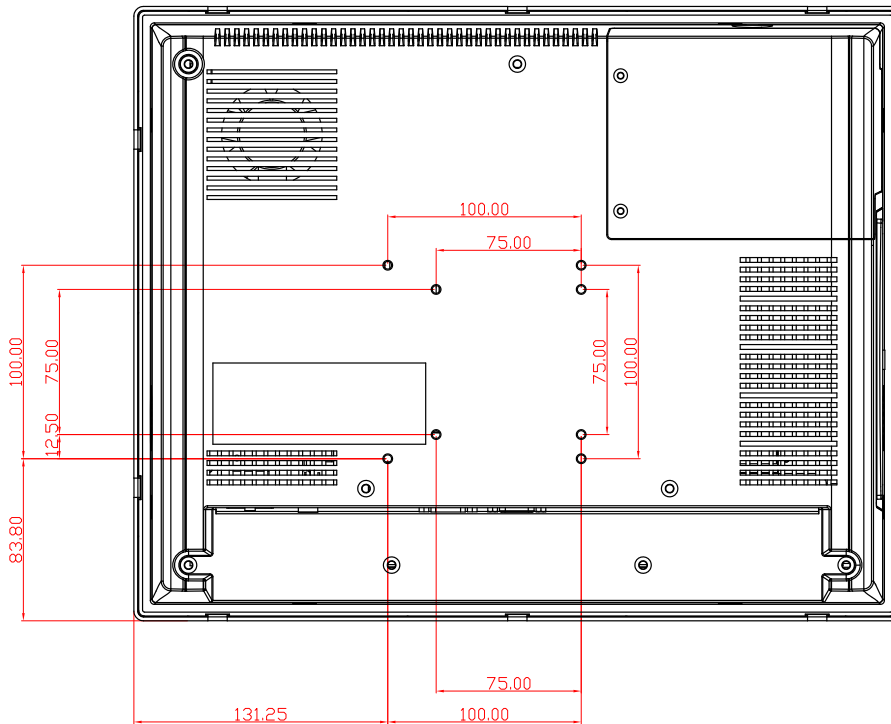
Figure 2.4 Rear View of the Panel PC
