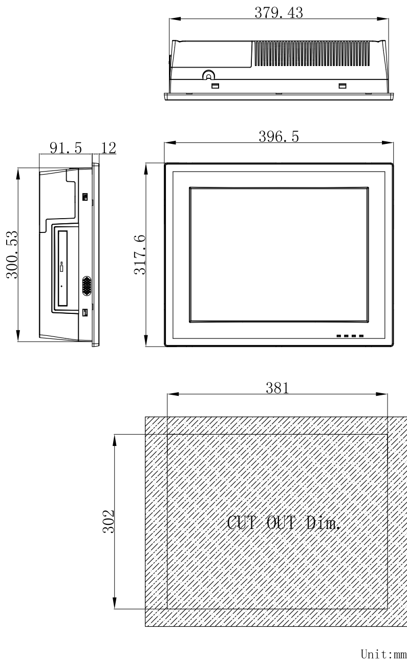
Figure 1.1 Dimensions of PPC-157T
