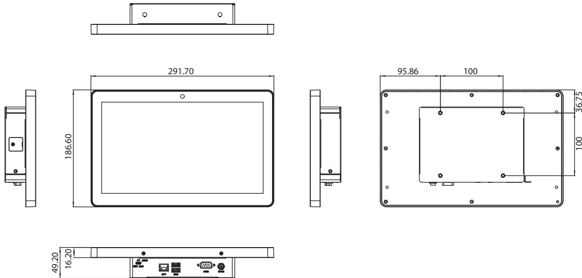
Panel Cutout Dimensions: 298.00 x 193.00 mm (11.73 x 7.60 in)
