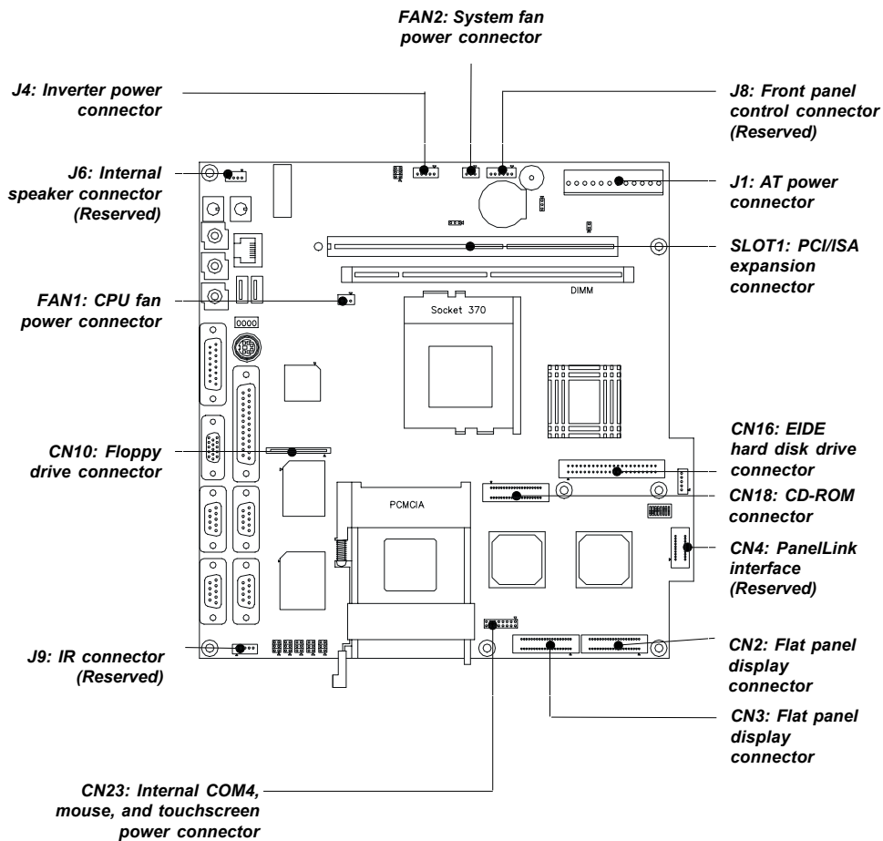
Figure 3-2: Locating connectors on the IPPC-9120/9150 motherboard
