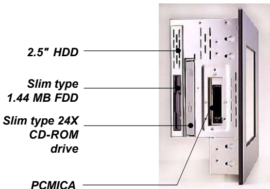
Figure 2-1: Side view
