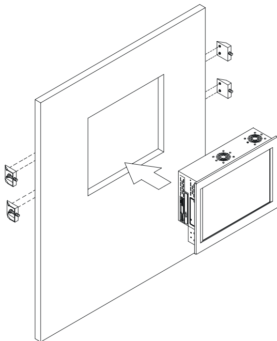
Figure 2-11: Panel mounting
