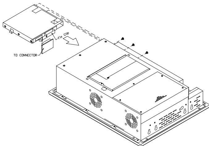
Figure 2-8: Removing the back case screws
