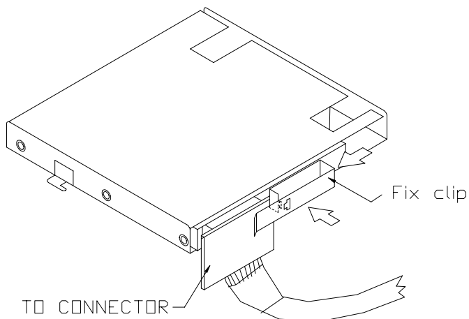
Figure 2-9: Attaching the connector to the CD-ROM
