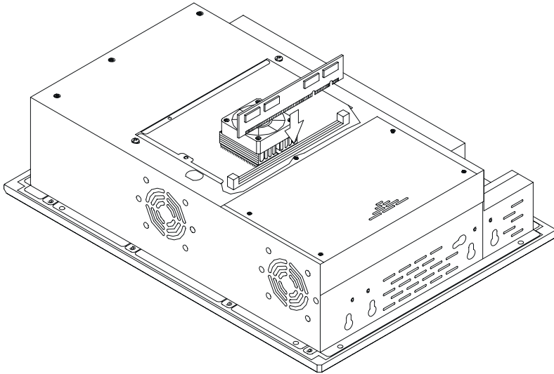
Figure 2-3: Installing SDRAM
