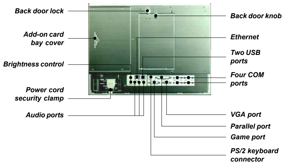
Figure 2-2: Rear view
