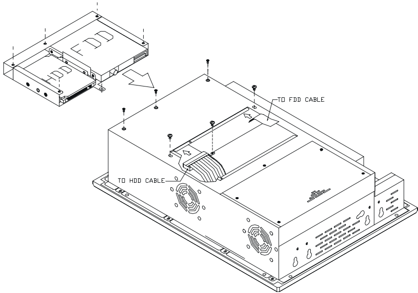
Figure 2-5: Removing the back case screws
