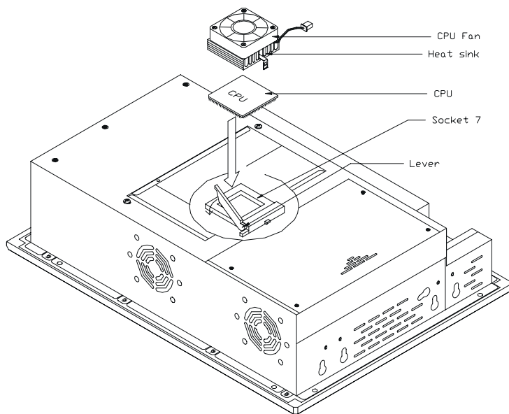
Figure 2-4: Installing a CPU
