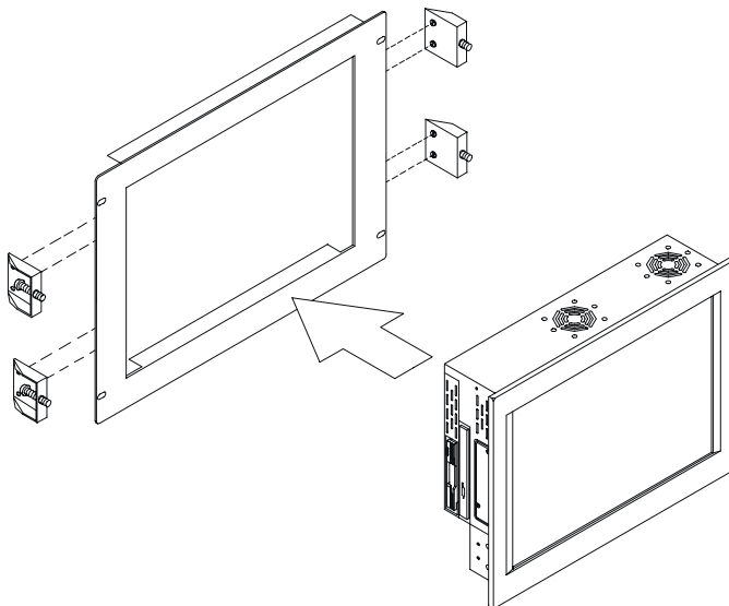
Figure 2-12: Mounting the IPPC-9120/9150 Series into a frame
