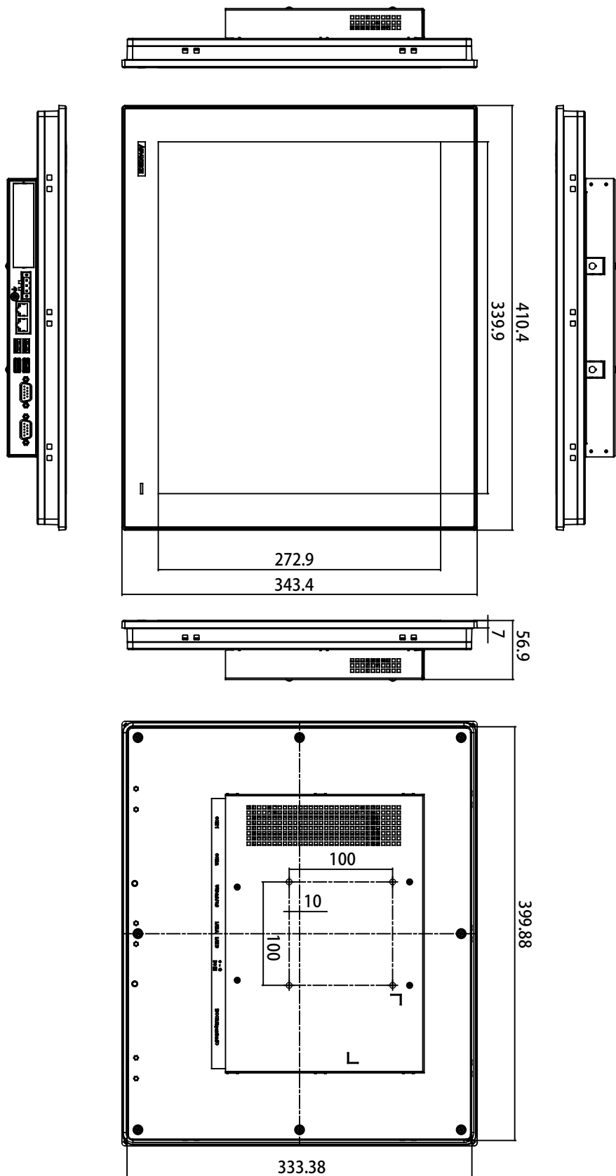
Figure 1.4 TPC-1751T Dimensions
