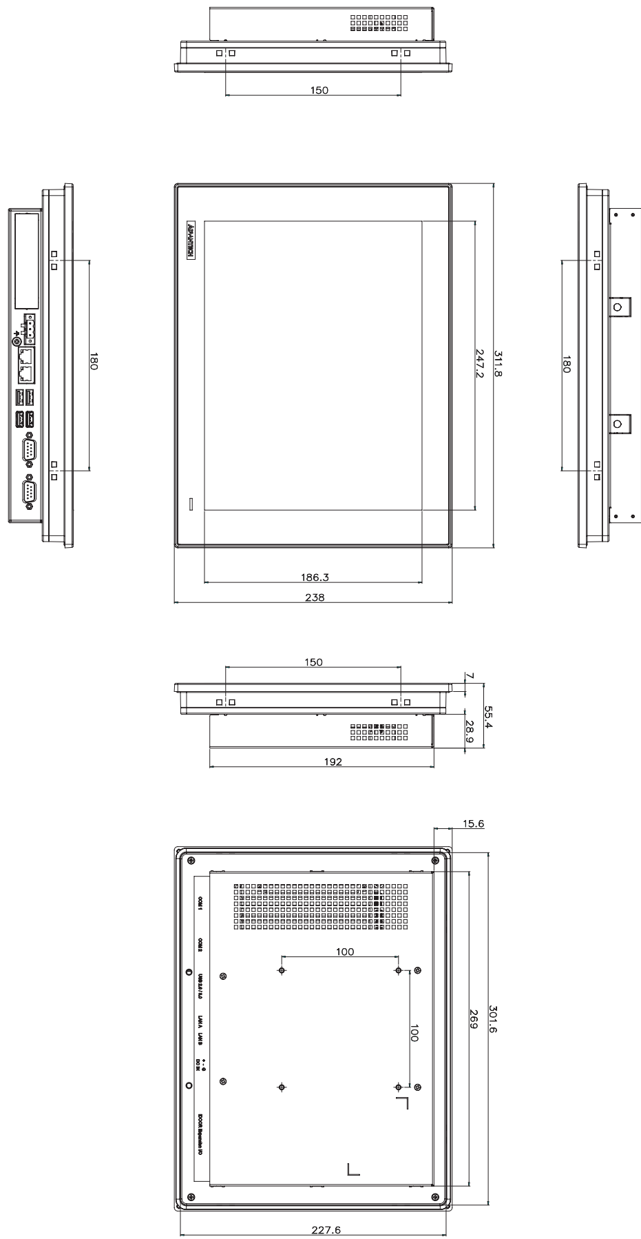
Figure 1.2 TPC-1251T Dimensions
