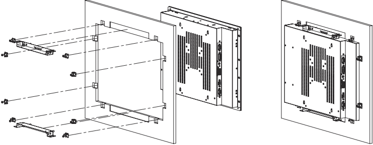
Figure 2.2: Panel Mounting (Cutout Dimensions: 447.5x329.5)
