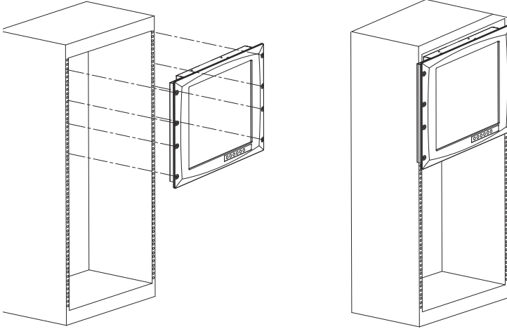
Figure 2.3: Rack Mounting
