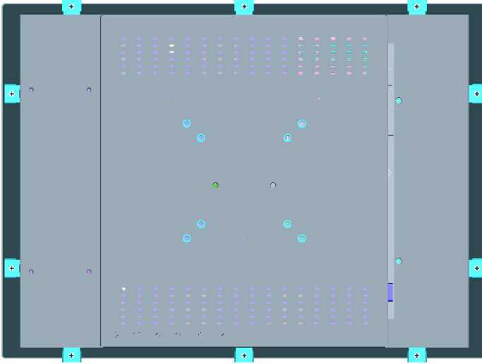
Figure 2.2: Panel Mounting
