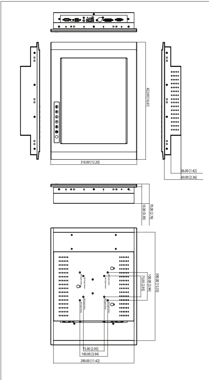
Figure 1.1: FPM-3151G Dimensions
