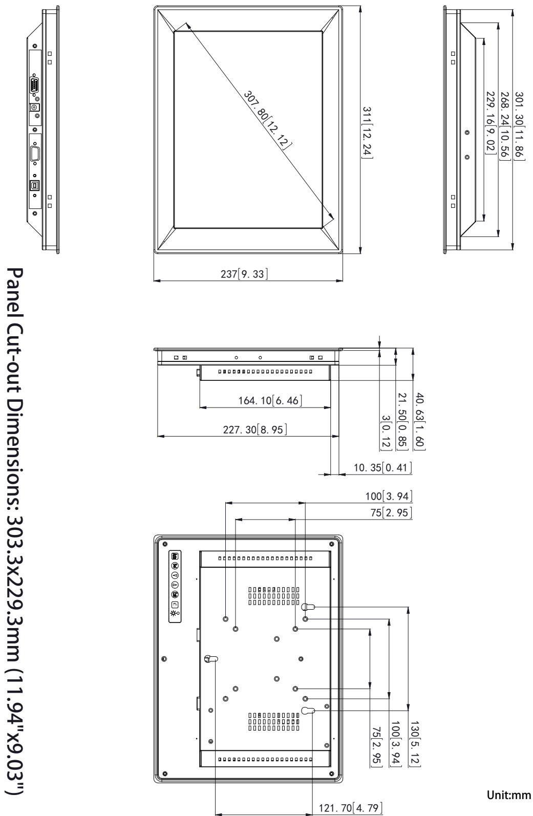
Figure 1.1 FPM-2120G Dimensions
