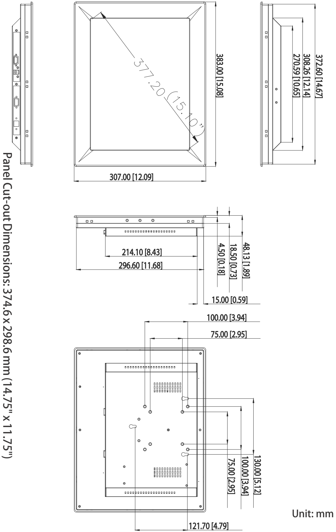
Figure 1.2 FPM-2150G Dimensions
