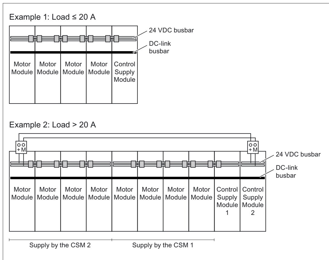
Figure 5-22 24 VDC division
