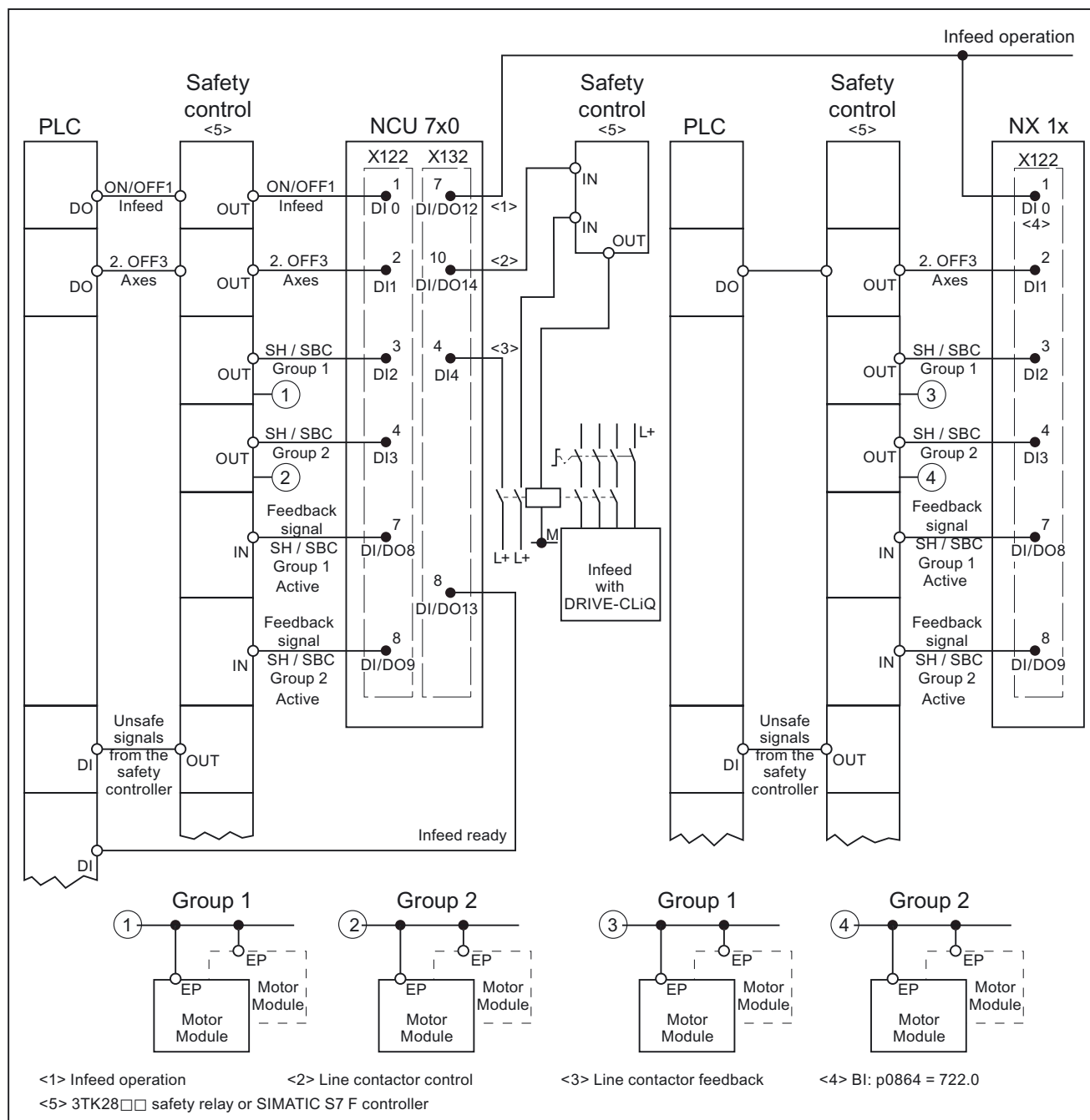
Figure 6-4 Infeed with DRIVE-CLiQ (SLM/ALM 16 kW to 120 kW), use of a drive-integrated SH/SBC safety function by SINAMICS and line contactor with safe control
