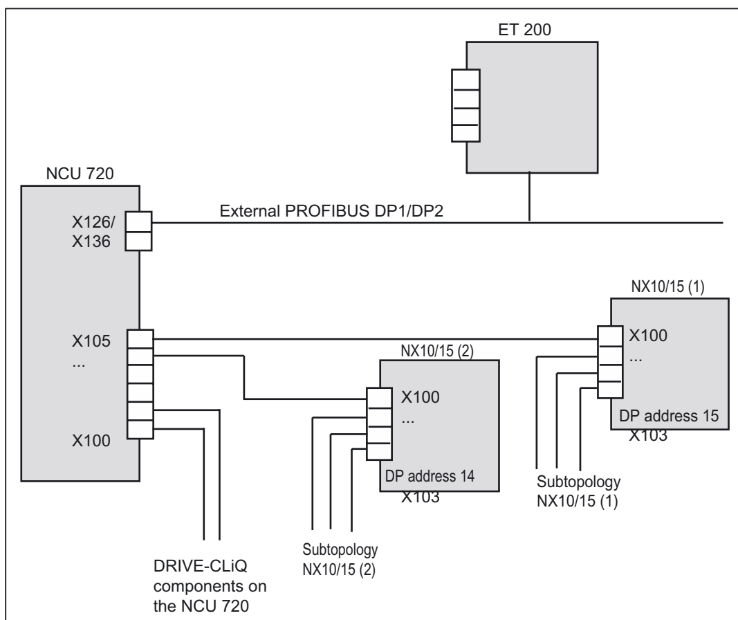
Figure 5-17 NX10/15 topology
