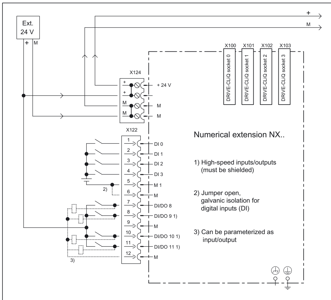
Figure 3-4 NX1x block diagram
