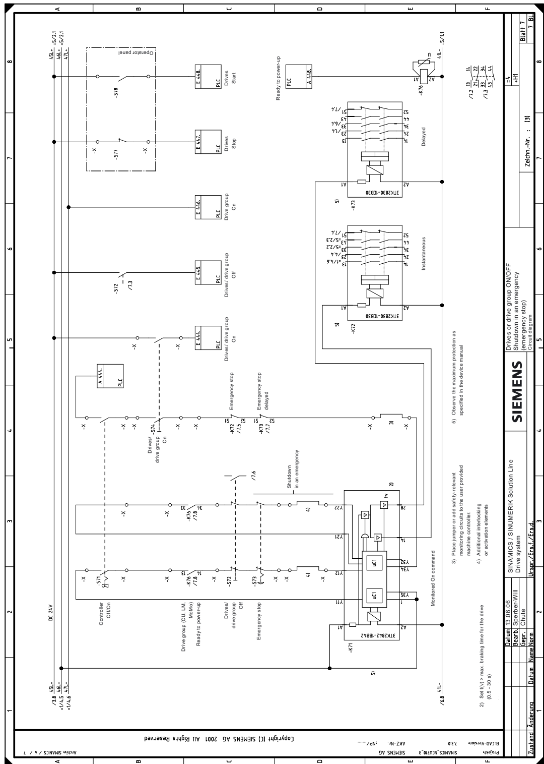
Figure 7-27 Circuit manual group =4, page 7
