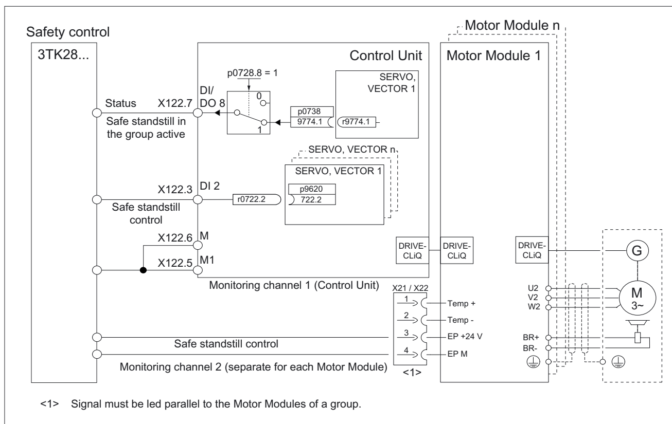
Figure 4-1 Terminals for "safe standstill"
