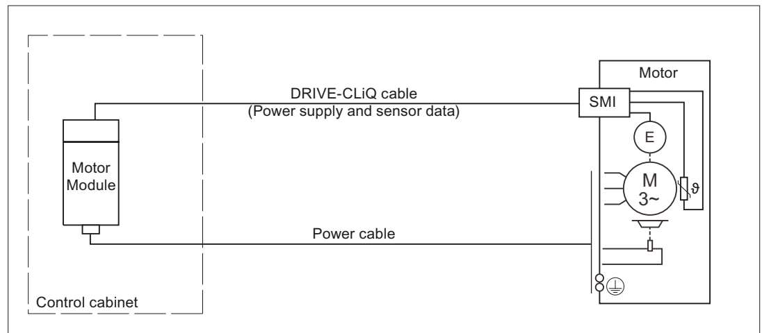
Figure 5-34 Sensor connection via a motor with a DRIVE-CLiQ interface
