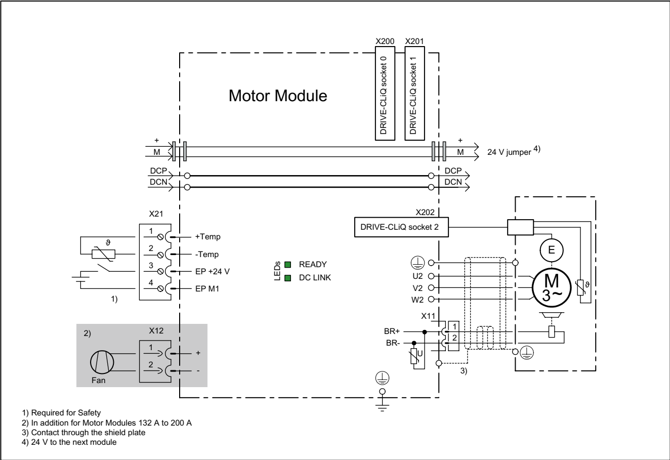
Figure 5-30 Example connection of Single Motor Modules 45 A to 200 A
