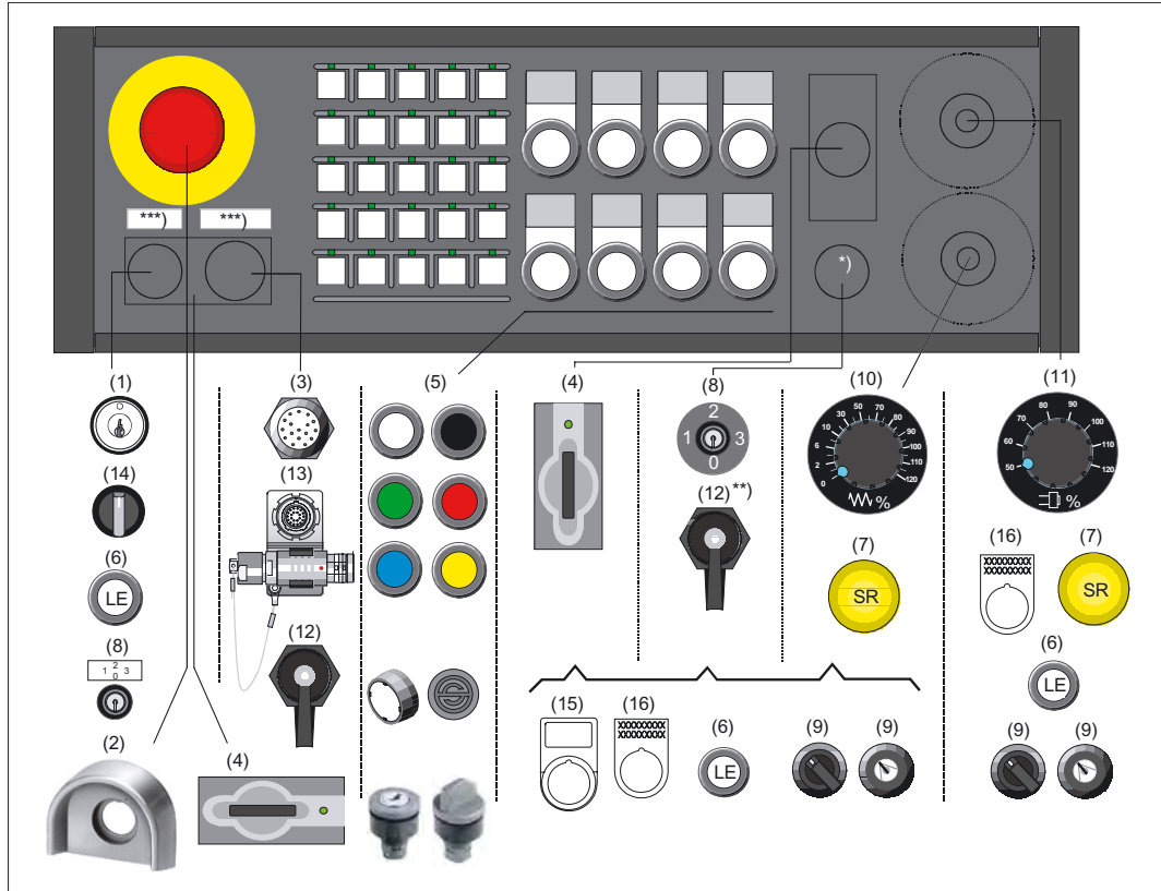
Figure 31-4 Special version MPP 483 S
