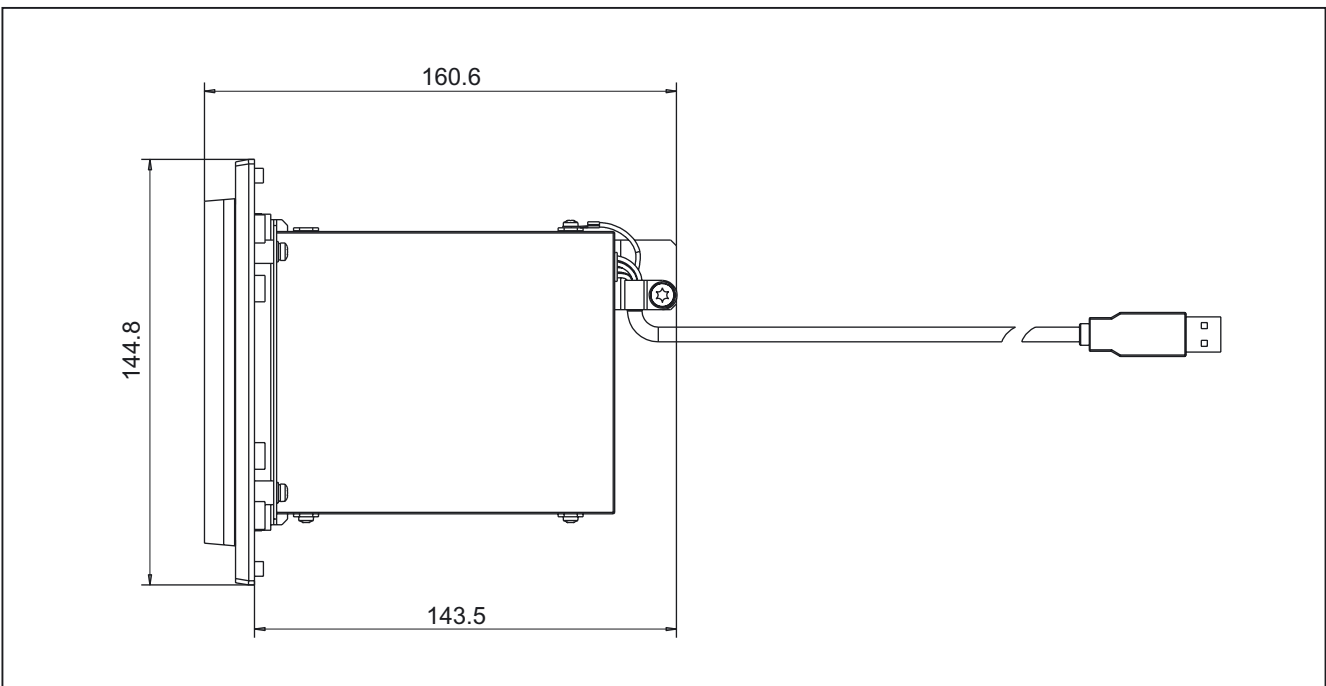
Figure 45-3 Top view
