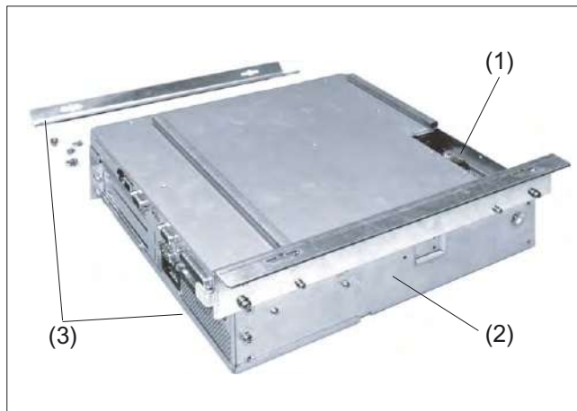
Figure 21-9 PCU with flat mounting brackets
