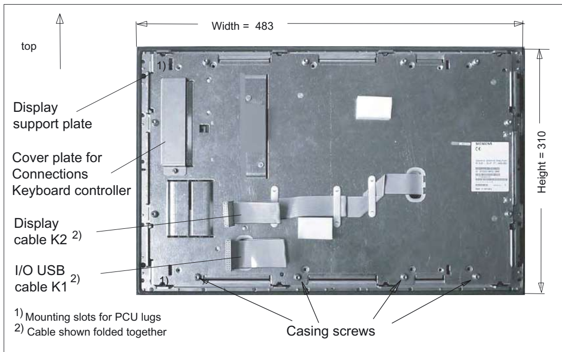
Figure 5-4 Rear side of operator panel front with position of interfaces and mounting slots
