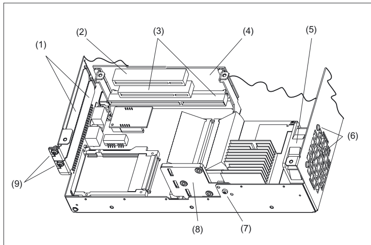
Figure 18-26 Expansion slots
