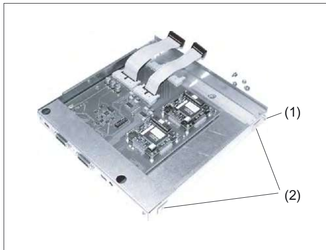
Figure 14-14 Videolink transmitter with connecting cables
