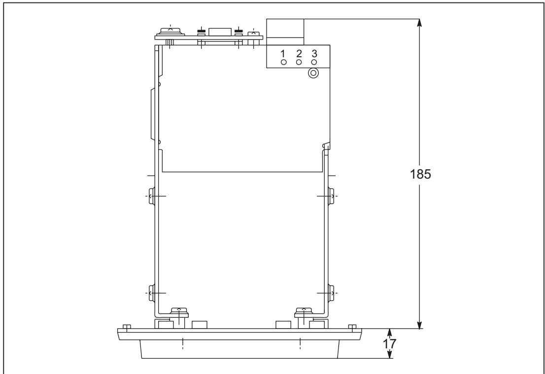
Figure 44-3 Top view
