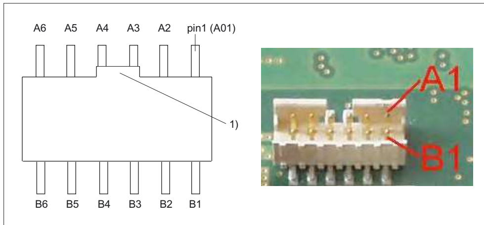
Figure 24-6 X51: Supply 2
