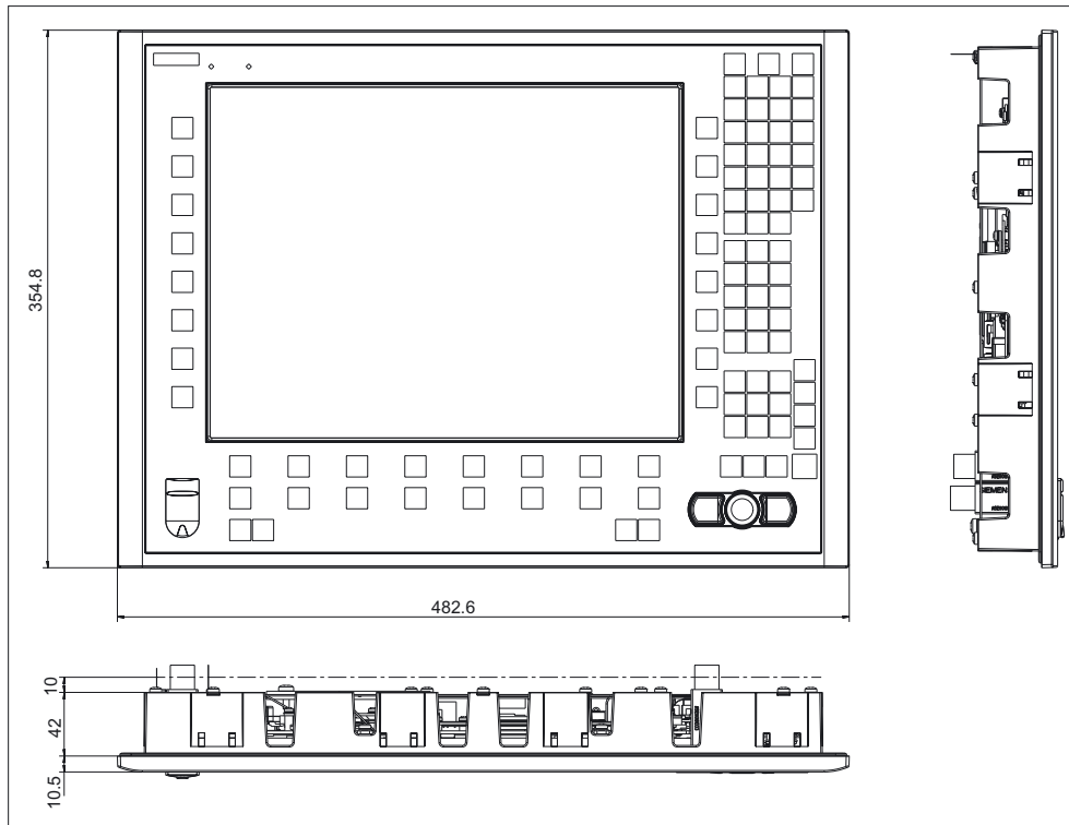
Figure 13-3 TP 015AT with TCU (integrated)
