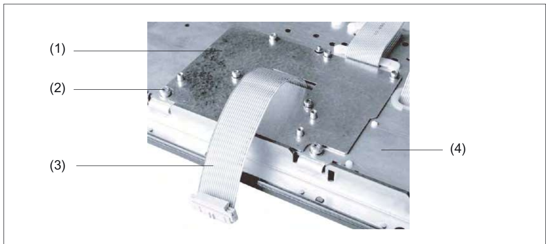
Figure 16-8 Installation of the direct control key module on the OP 012
