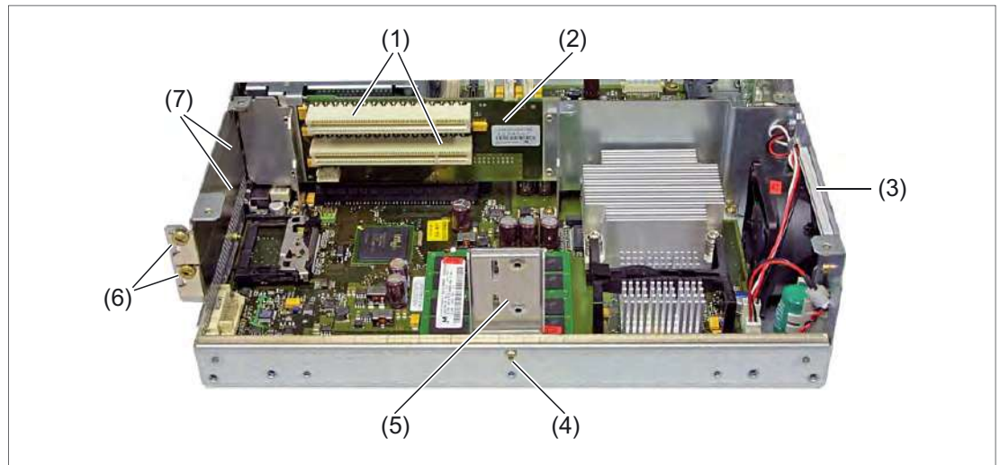
Figure 19-33 Expansion slots
