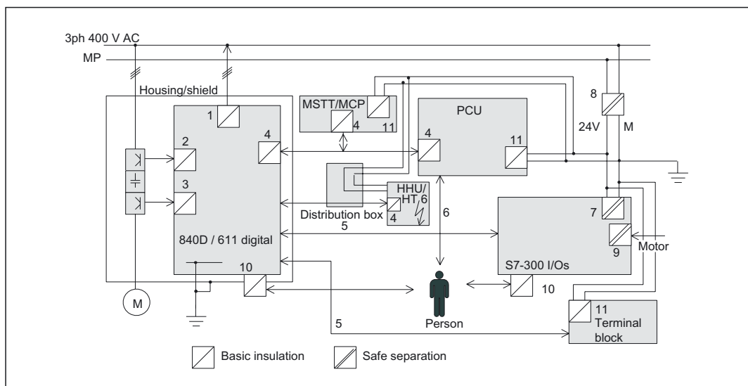
Figure 1-1 Safe isolation to EN 61800-5-1
