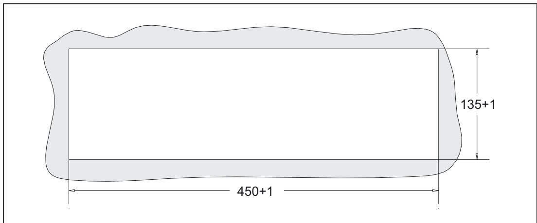
Figure 28-6 Panel cutout for machine control panel MCP 483
