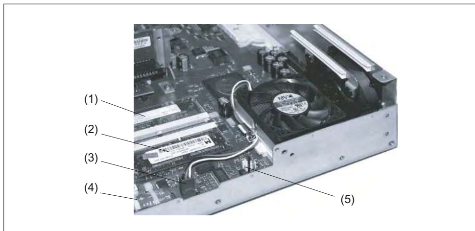
Figure 18-20 Main board PCU 50 > 500 MHz (cut-out) with location of RAMs and backup battery
