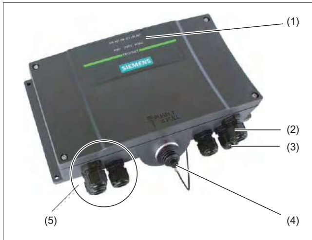
Figure 24-9 Terminal Box PN
