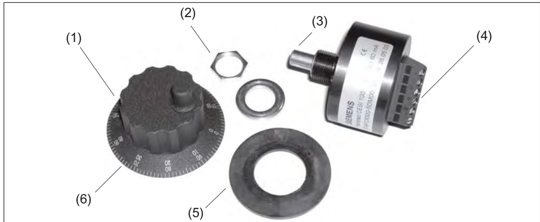
Figure 15-12 Mounting kit for handwheel
