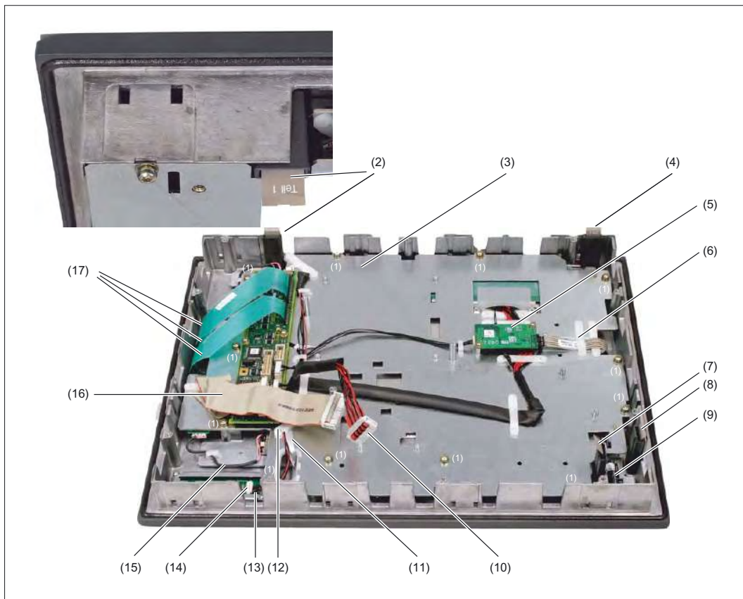
Figure 11-6 TP 015A housing open
