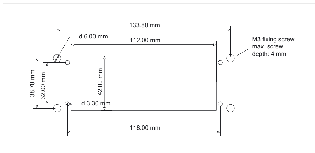
Figure 46-2 Panel cutout
