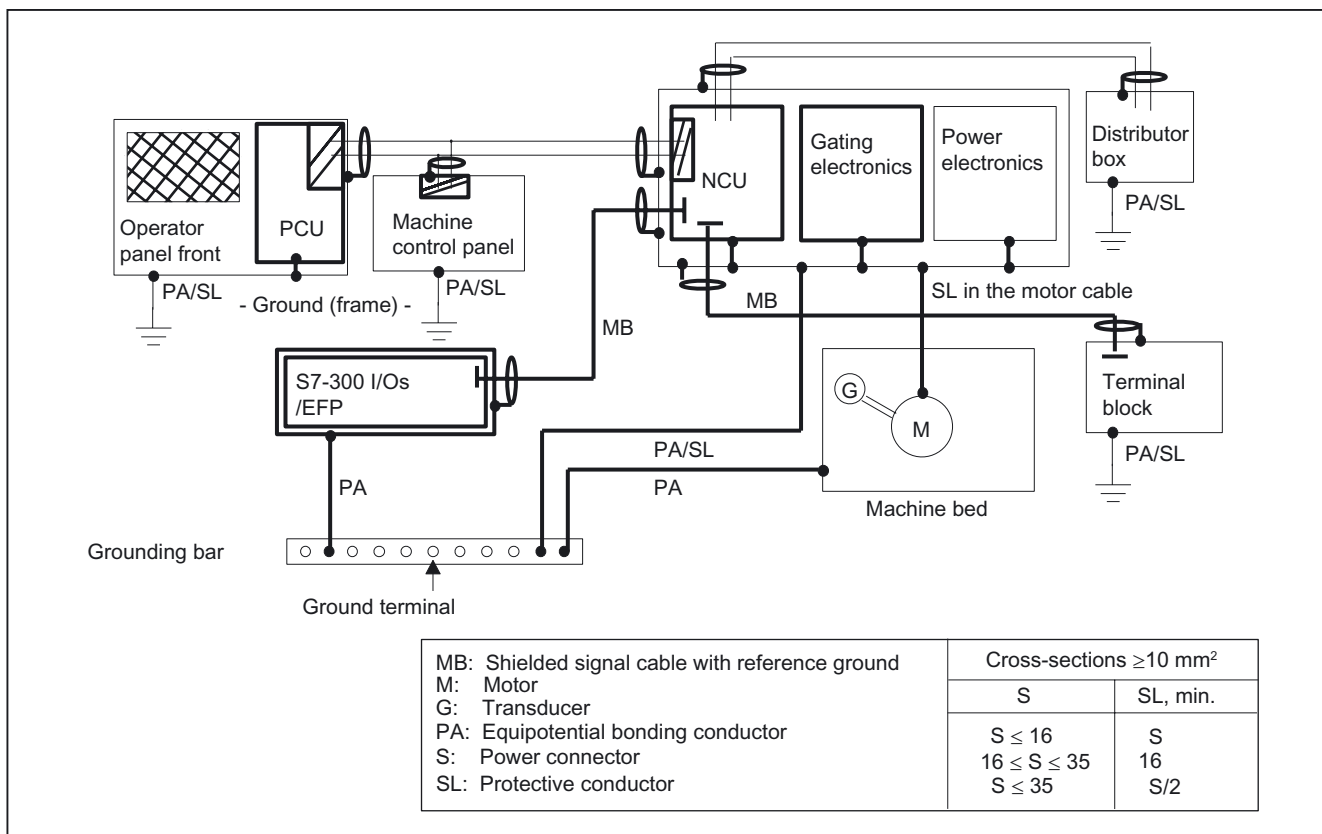
Figure 1-2 Grounding concept
