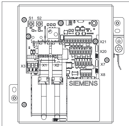
S1 / S2 DIP Fix switches (rotary coding switch)
