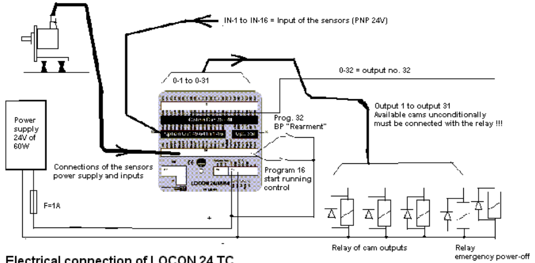
Electrical connection of LOCON 24 TC
