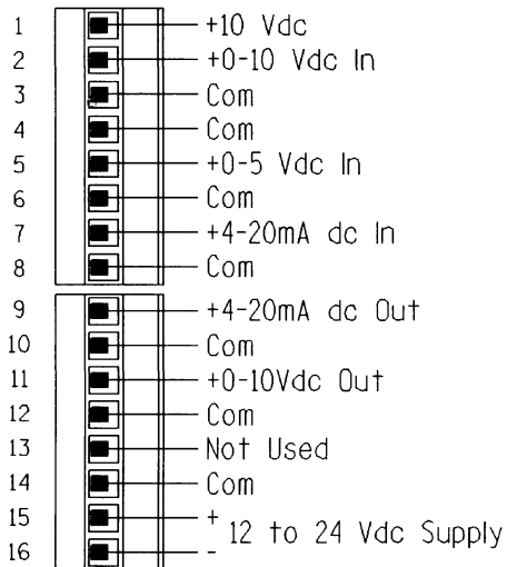
Figure 3, Analog and Power Supply Terminals
