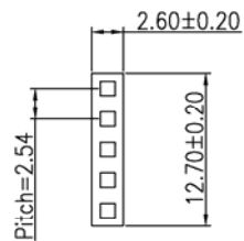
HOUSING
