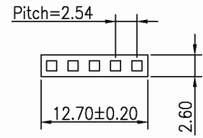
HOUSING
