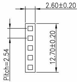
HOUSING
