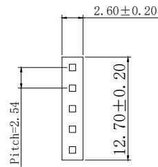
HOUSING
