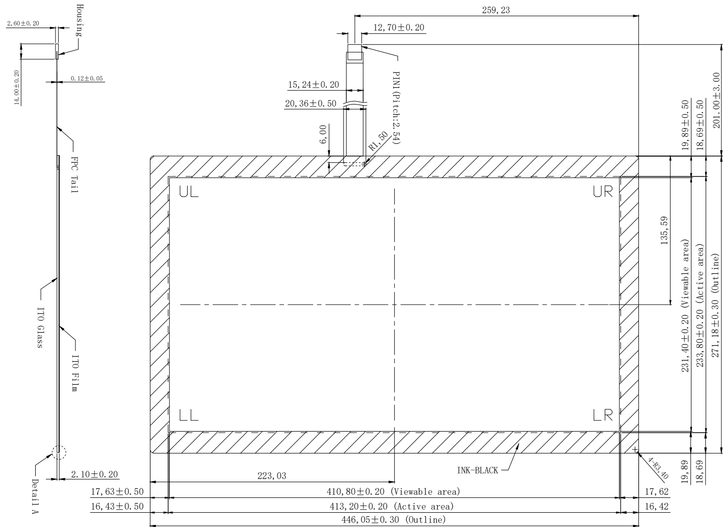
TOP VIEW
