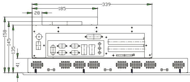
Appliance's rear view
