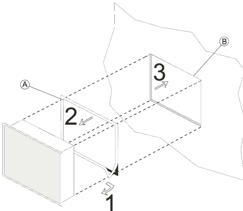
A Gasket B Installation cut-out
