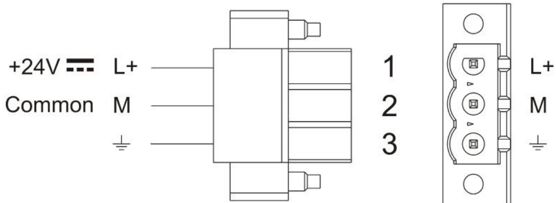
DC Power Connector, Female - R/C Terminal Blocks (XCPR2), manufactured by Weidmüller Inc., Cat. No. BLZ 5.08, torque 4.5 lb-in
