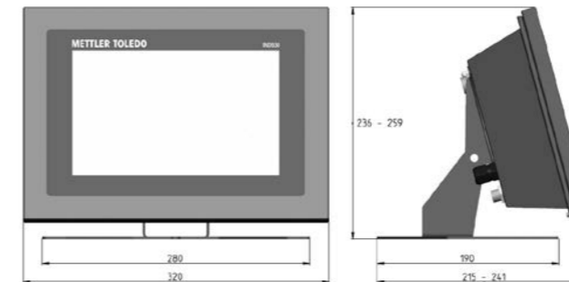
IND930 – desk version
