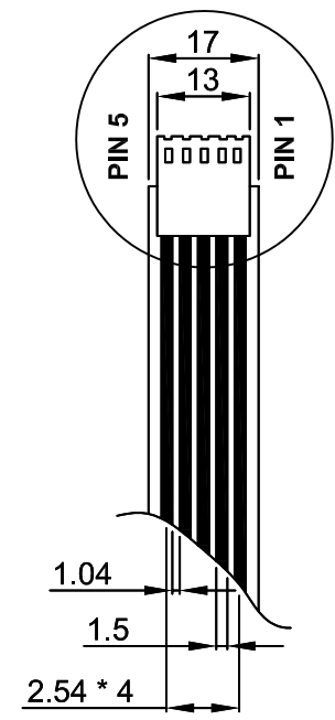
DETAIL A
