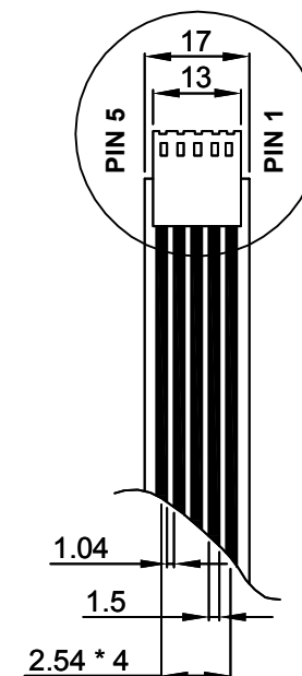
DETAIL A
