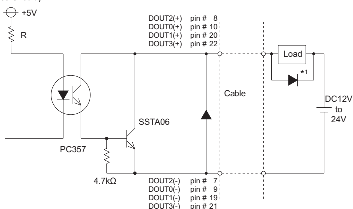
( Interface Circuit )
