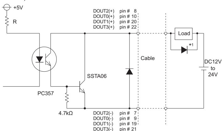
( Interface Circuit )
