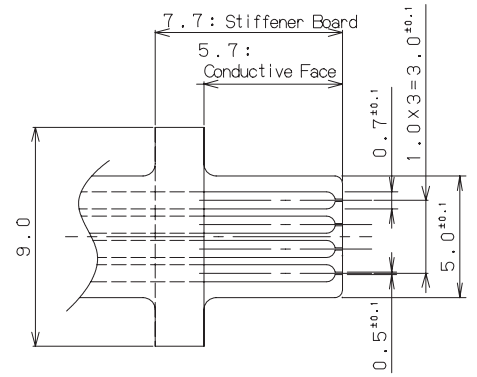
Conductive Face (導通面) FFC-Type Cable
