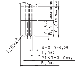
Conductive Face (導通面) FPC-Type Cable
