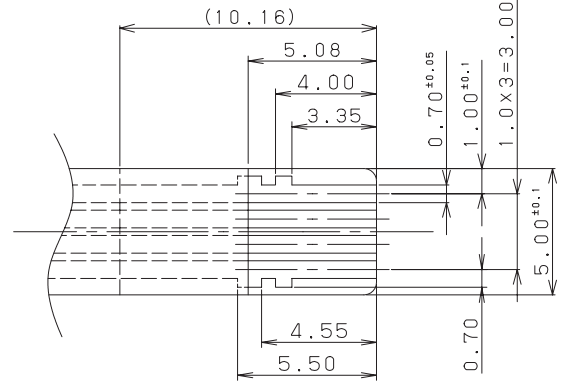
Conductive Face (導通面) FFC-Type Cable
