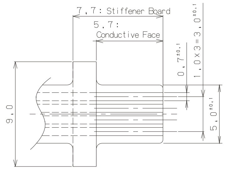
Conductive Face (導通面) FPC-Type Cable
