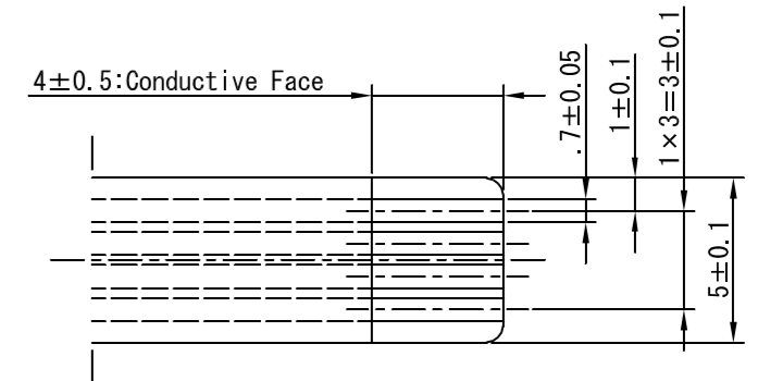
Conductive Face (導通面) FPC-Type Cable
