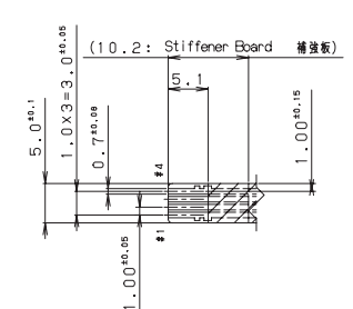
Conductive Face (導通面) FPC-Type Cable
