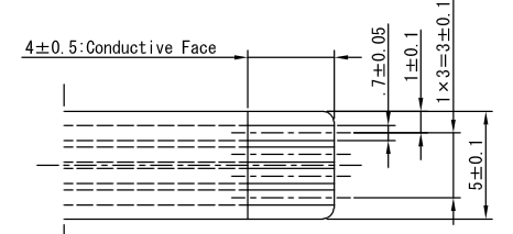
Conductive Face (導通面) FPC-Type Cable
