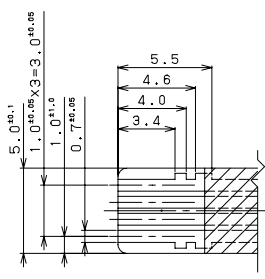
Conductive Face (導通面) FPC-Type Cable
