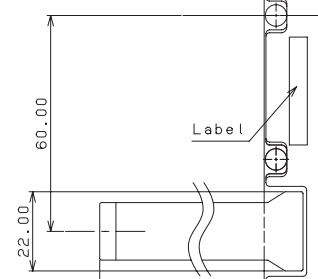
Contact Sectioning View (コネクタ断面図)
