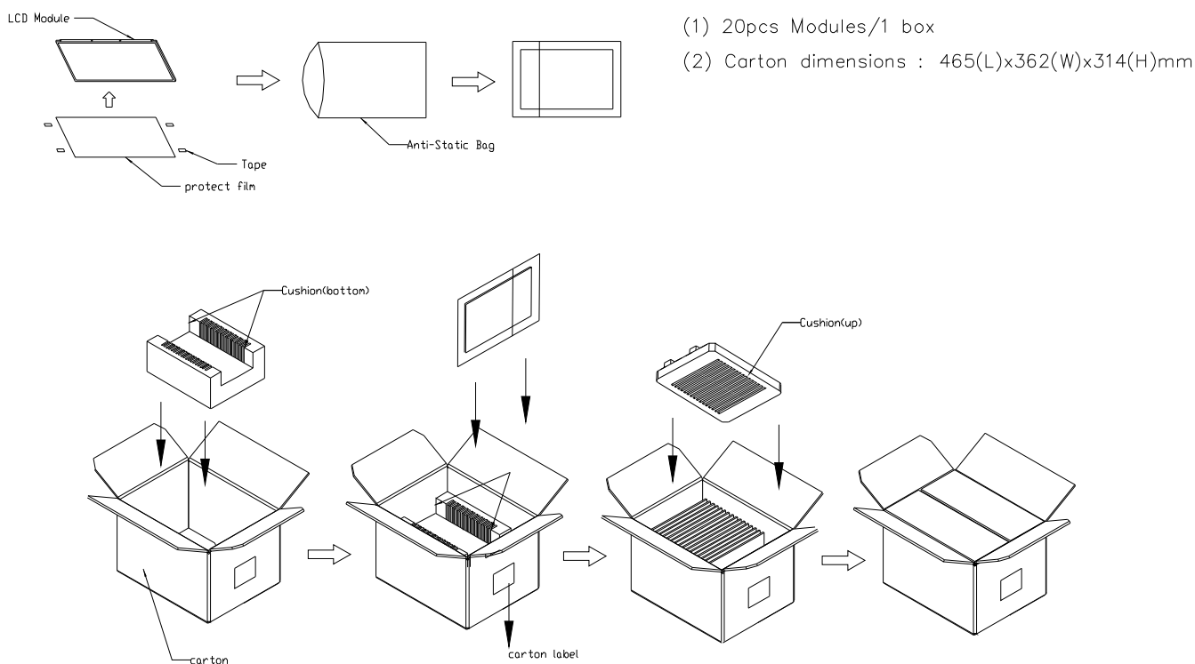
Figure. 7-1 Packing method
