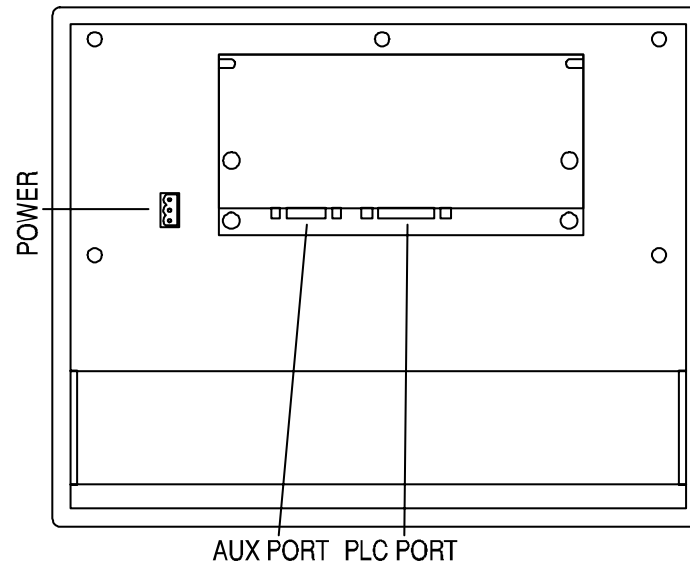
Figure 37 - Connectors
