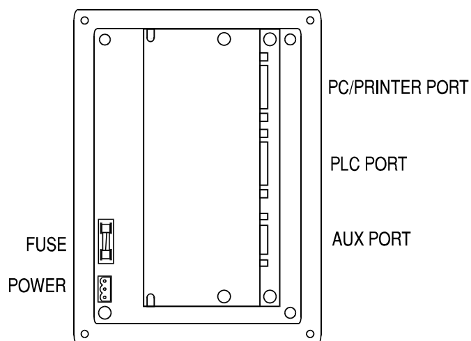
Figure 25 - Connectors
