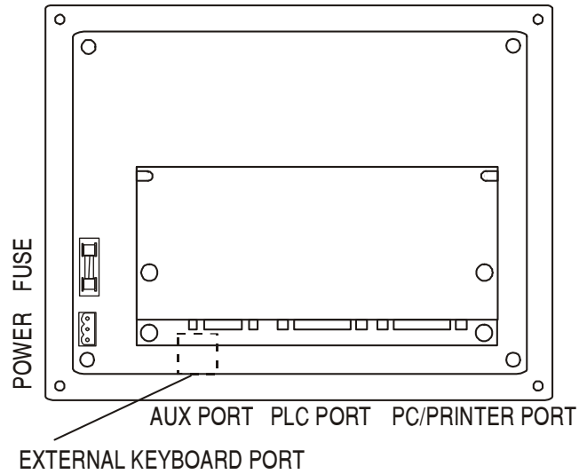
Figure 29 - Connectors
