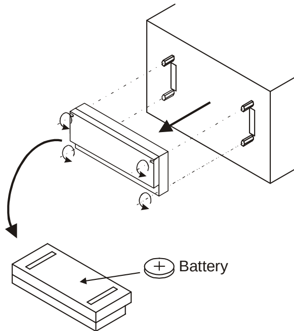
Figure 48 - battery replacement
