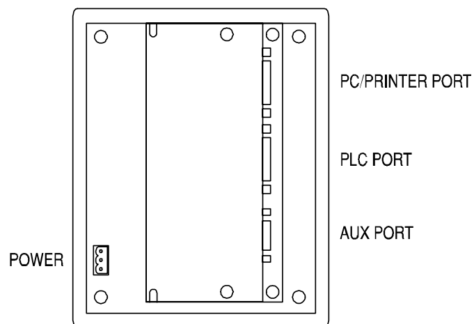
Figure 27 - Connectors
