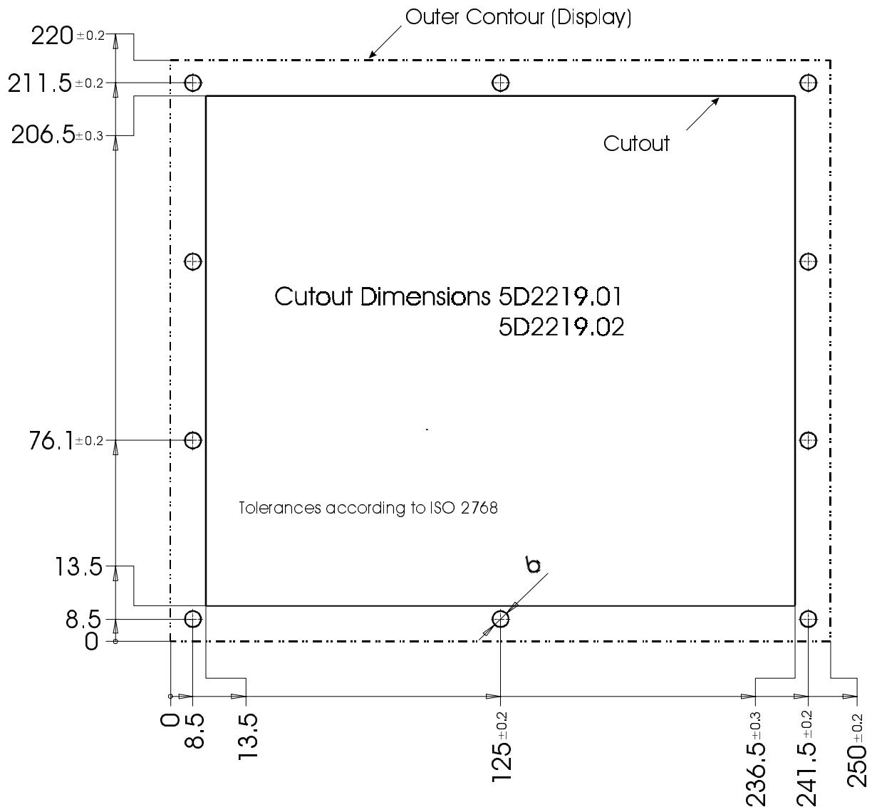
Image 69: Door Mount Installation, Display Unit 5D2219.01, 5D2219.02
