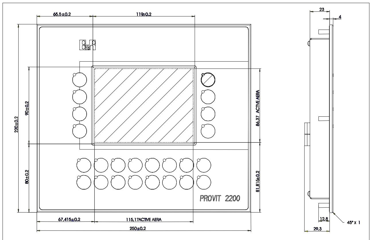
Image 68: Display Unit 5D2219.01, 5D2219.02
