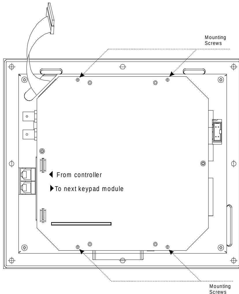
Image 70: Display Unit 5D2219.01 and 5D2219.02 - Mounting the Controller
