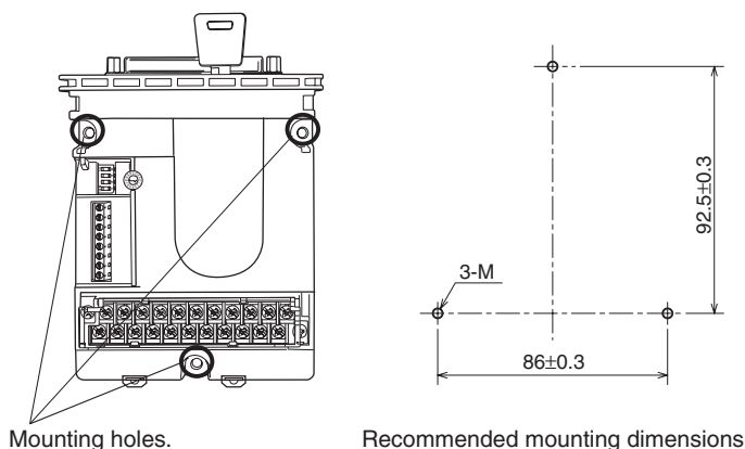
Mounting holes.
