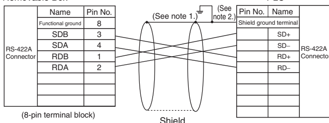
RS-422A Terminal Block on Removable Box
