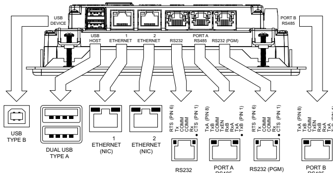
CR3000 07/10/15 PORT PIN OUTS
