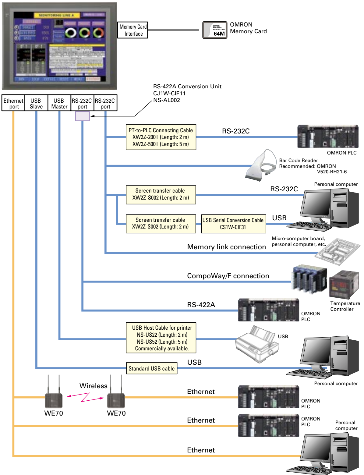
System Configuration Diagram
