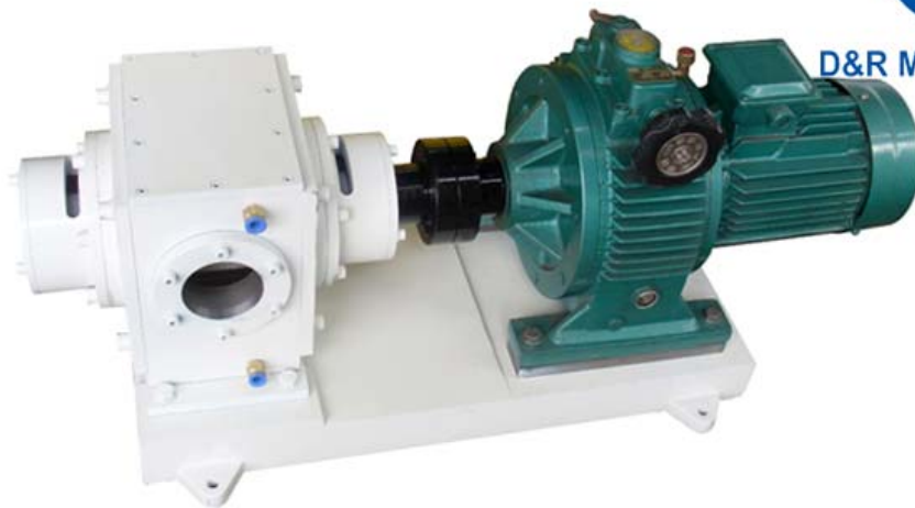
DR-SJB80Y chocolate pump
