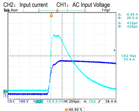
INPUT=230VAC/50HZ @ FULL LOAD
