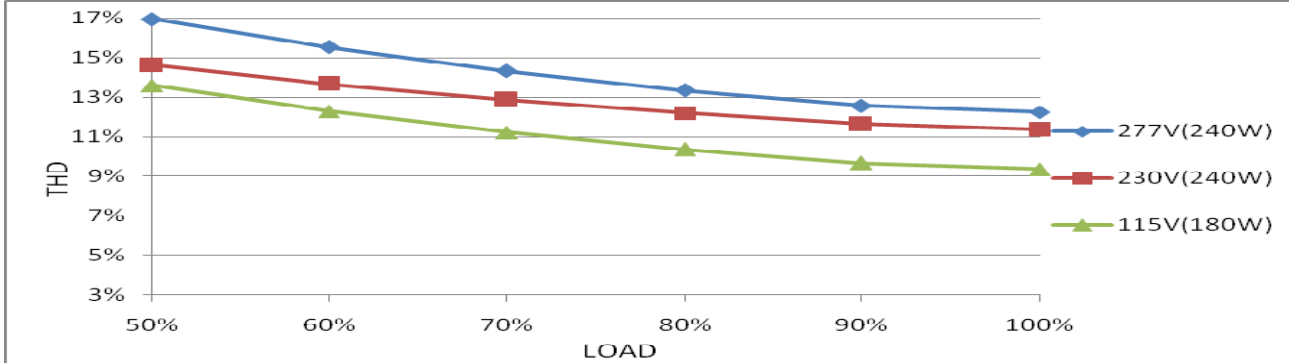
THD vs LOAD
