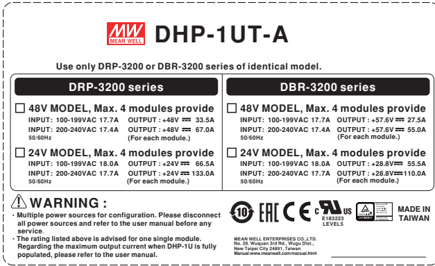
Figure 1-3: Safety label of DHP-1U
