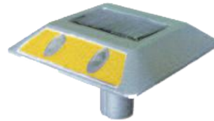
ATRS-2007 Name: Solar road stud Size: 132X122X75mm
