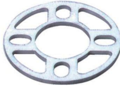
Part#: WS-101 Description: 4 Holes on 98-120mm Thickness:8mm I.D: 75.5mm O.D: 151.51mm
