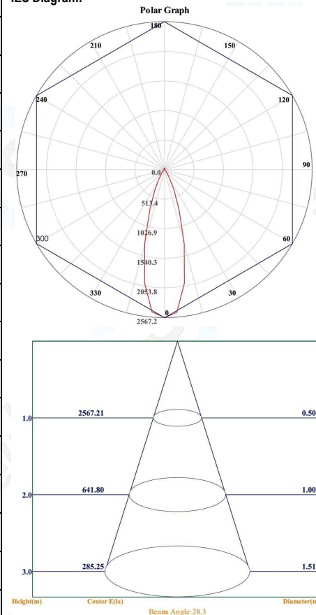
IES Diagram:
