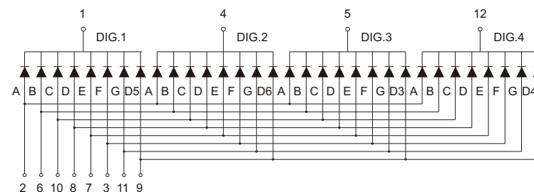
Common Anode NFD-4041Dx
